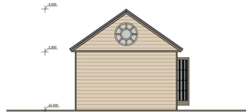
SOUTH-WEST ELEVATION
