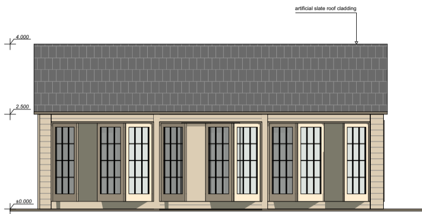
HOUSE SIDE/FRONT ELEVATION
