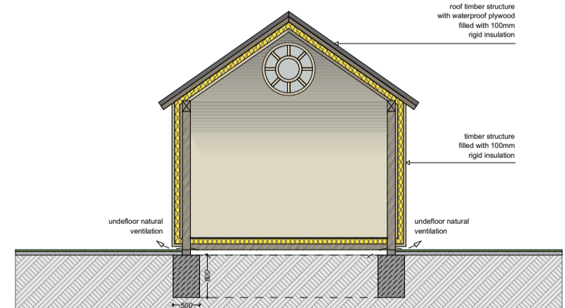
PRINCIPAL CROSS SECTION S1 AC-01
