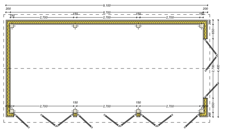
GENERAL FLOOR PLAN
