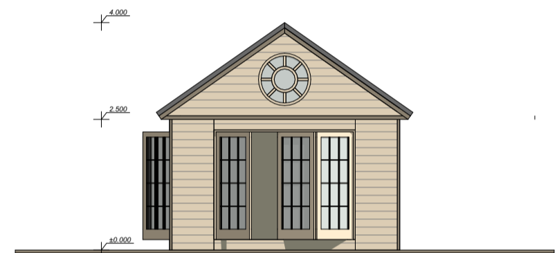
NORTH-EAST ELEVATION
