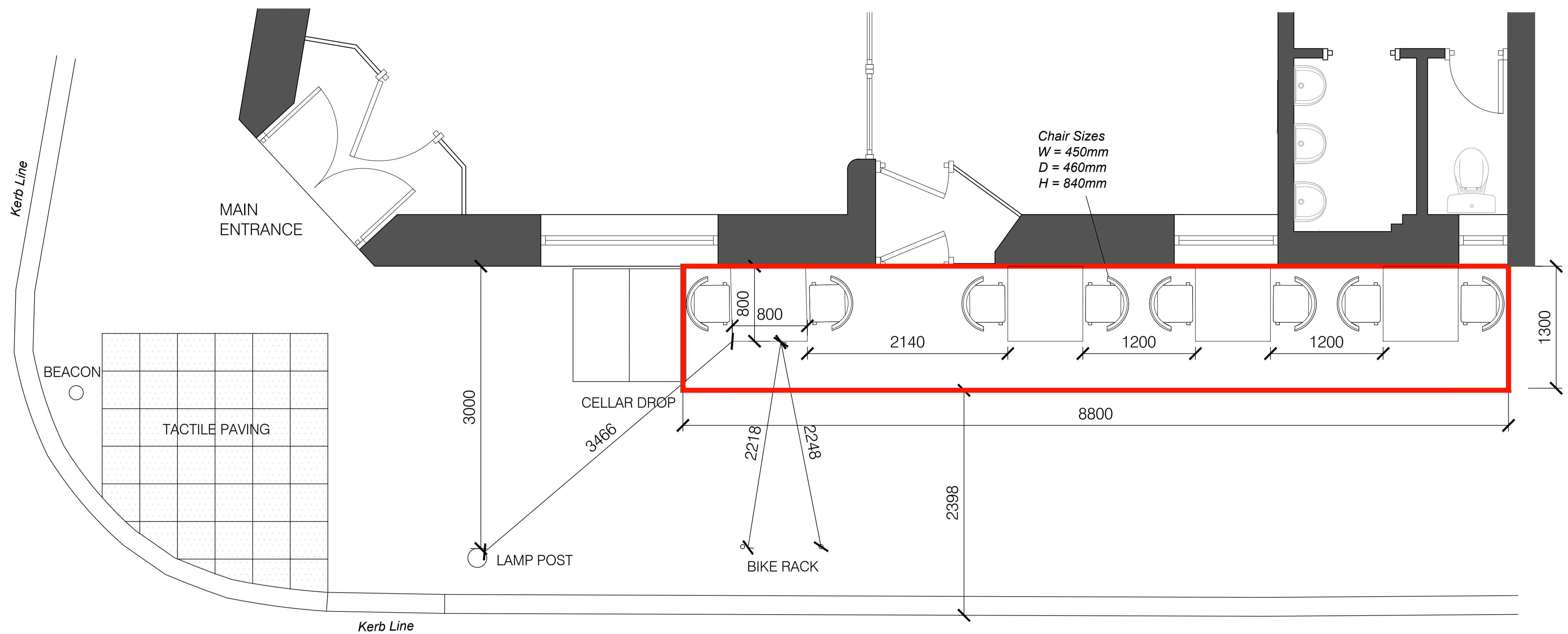
PROPOSED PAVEMENT LAYOUT
