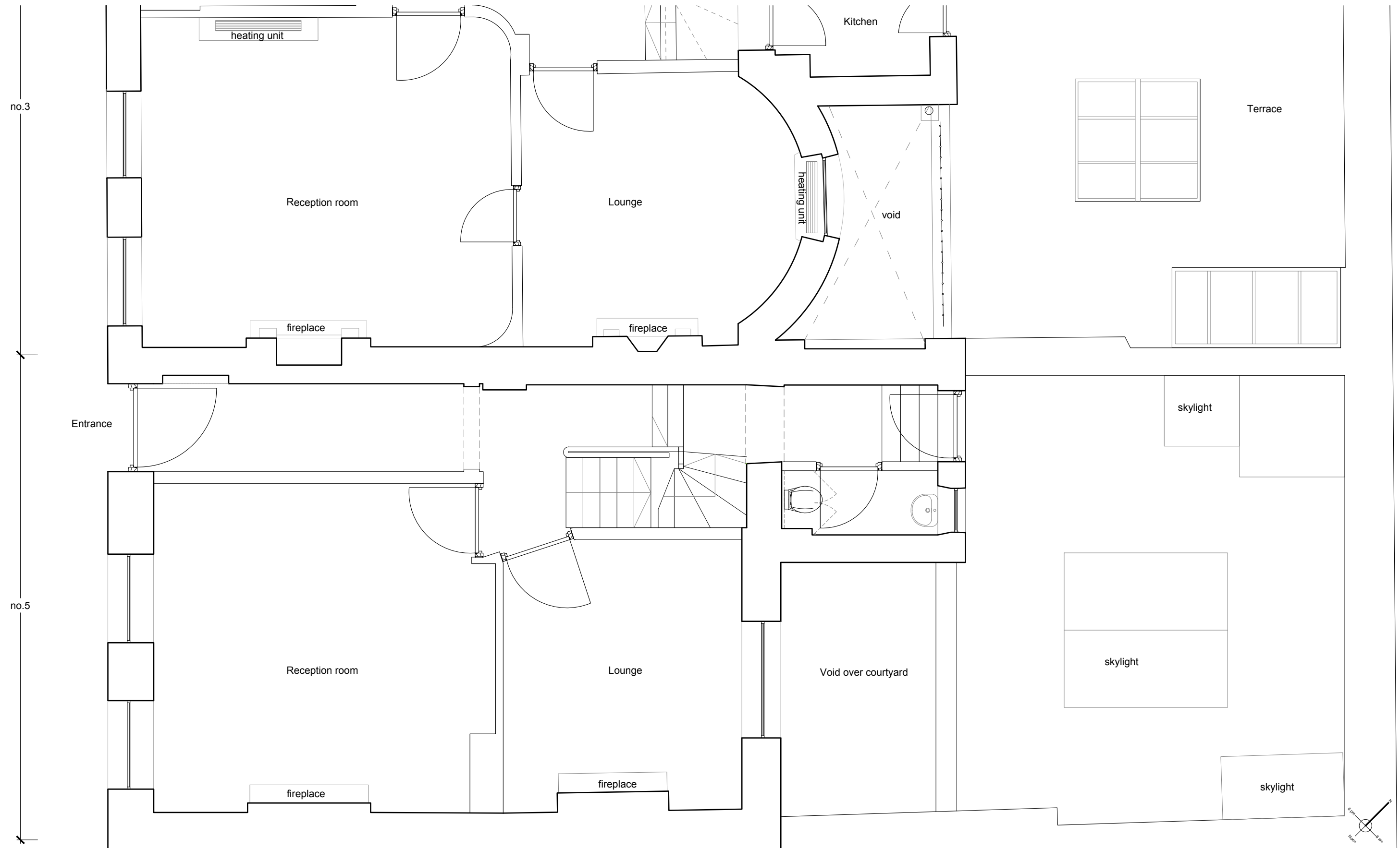
1 Existing Ground floor plan Scale 1:50
