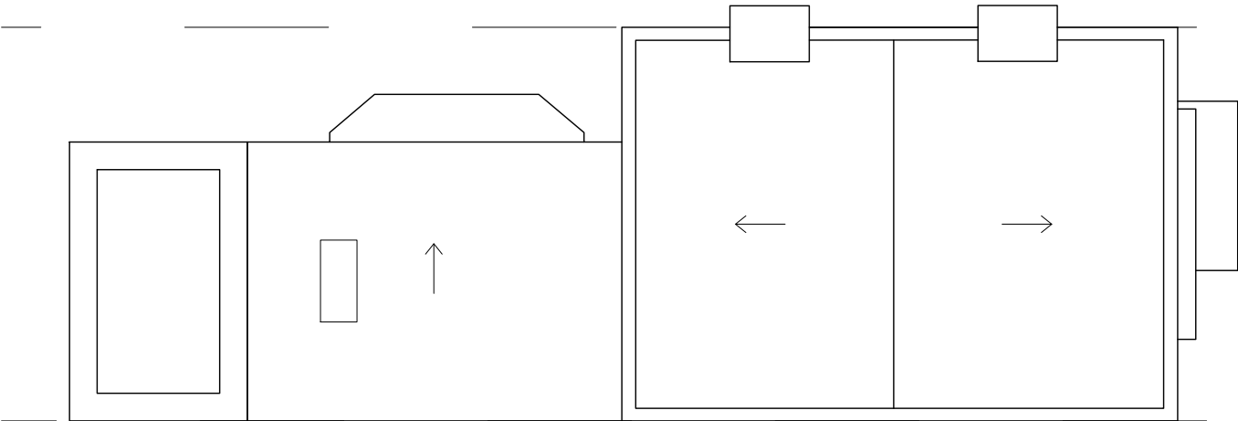
ROOF PLAN - PROPOSED
