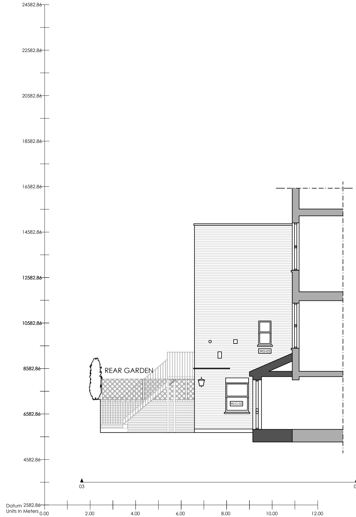
ELEVATION 3 (FLANK)
