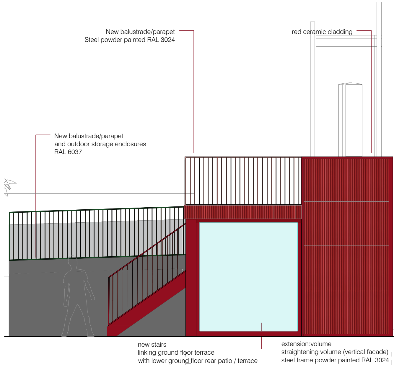
MAIN BUILDING - side (West) Elevation - proposed
