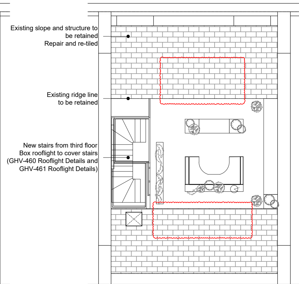
3 Proposed Roof Plan GHV 1:100 @ A3
