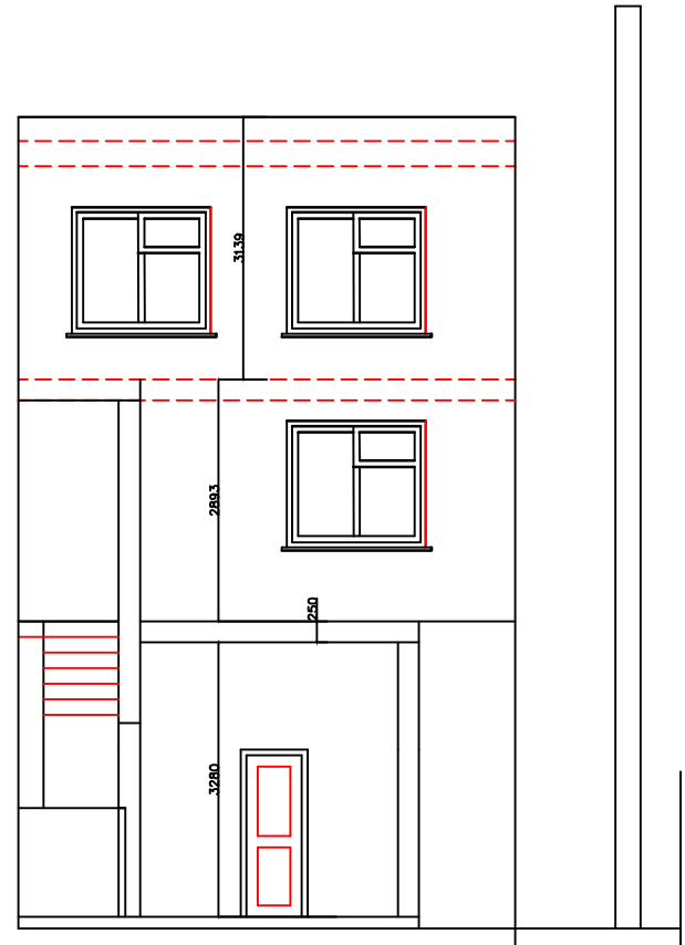
Sectional Elevation A - A
