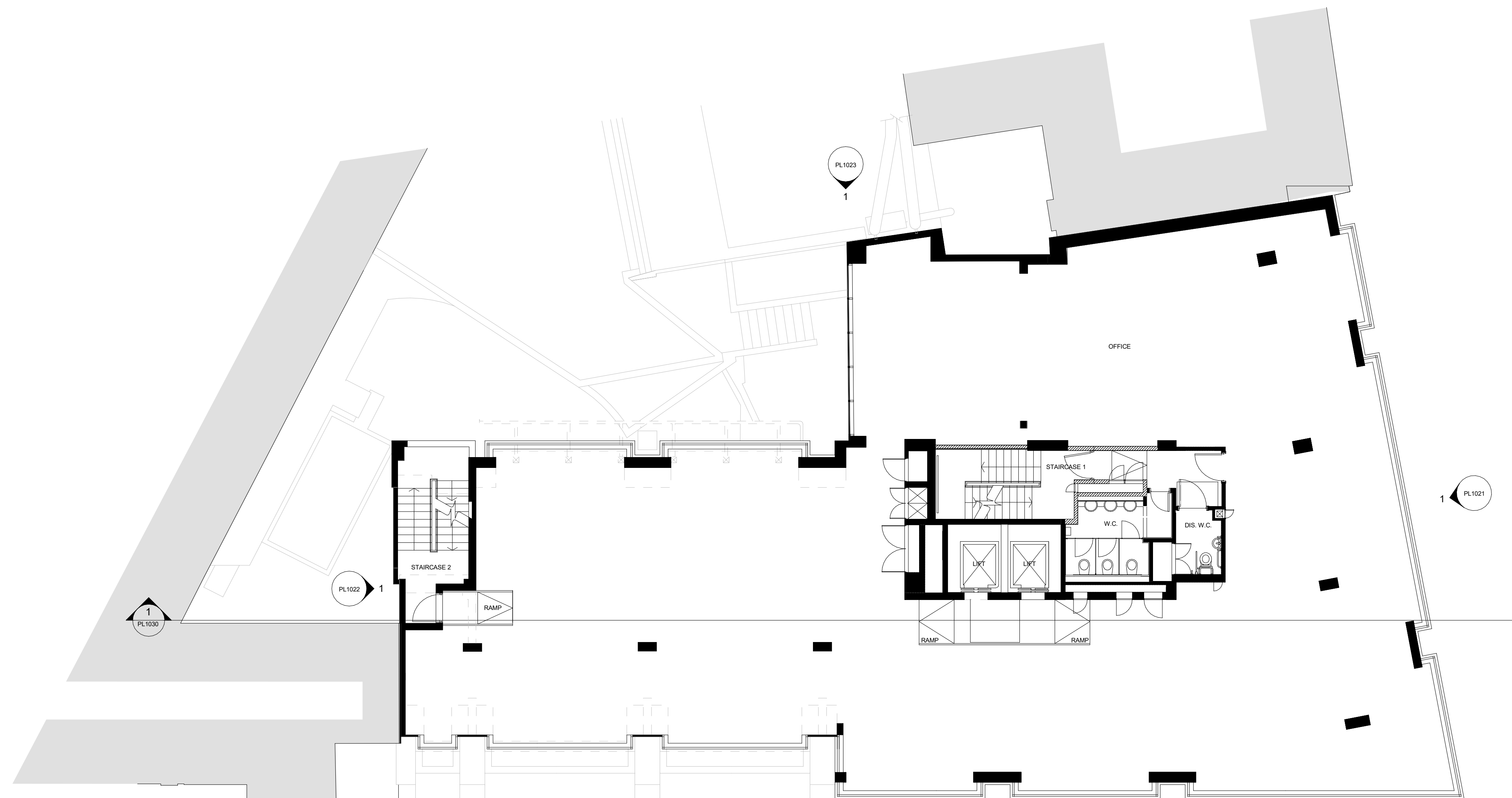
1 04 - Fourth Floor 1 : 100
