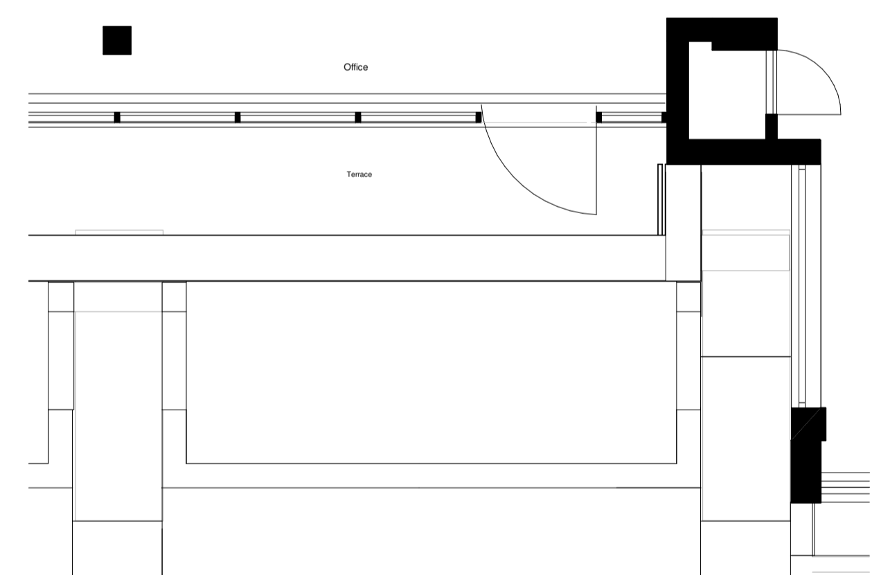
6 Fifth Floor Level - Gate/Terrace Detail 1 : 50
