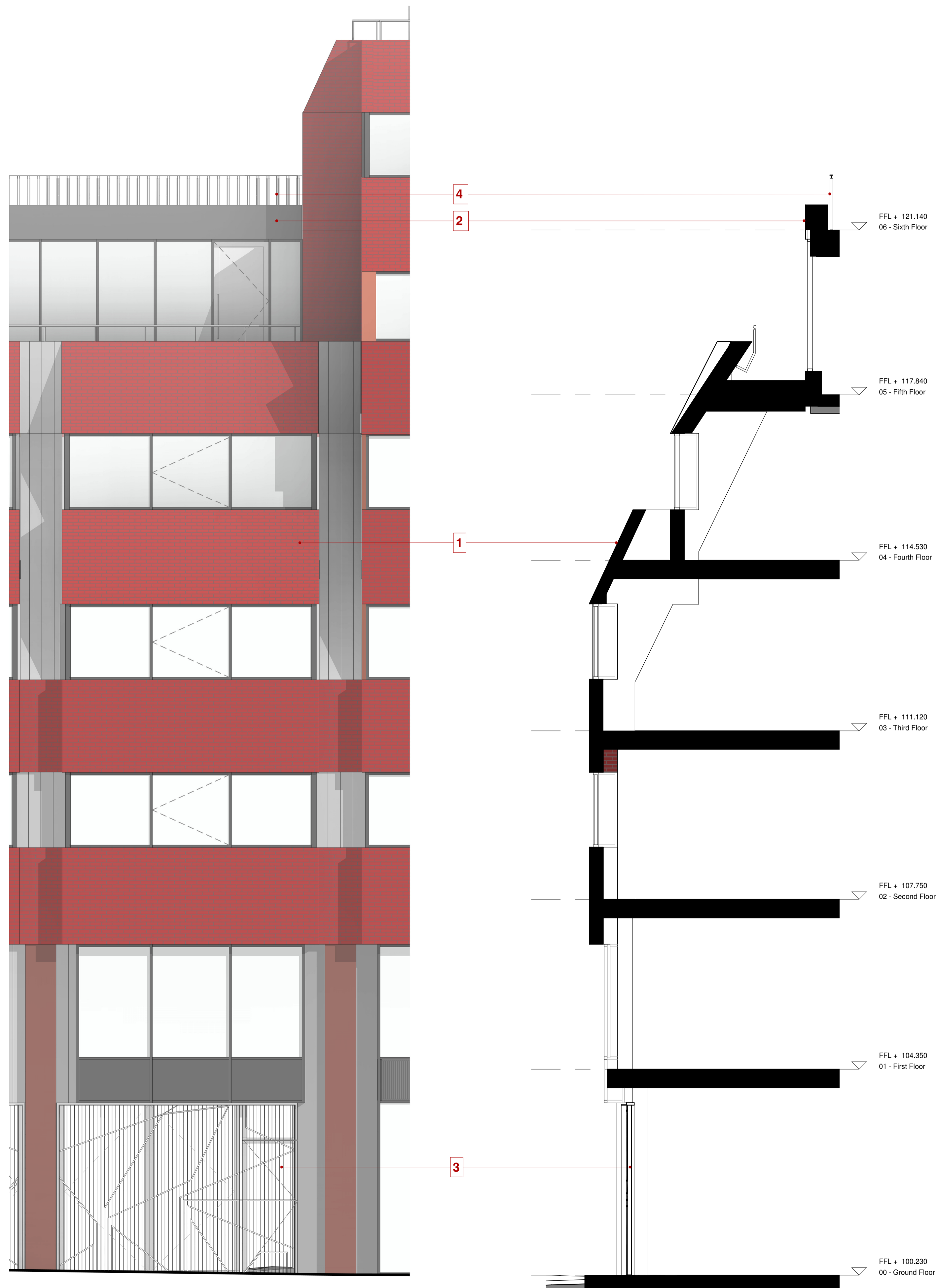
1 Proposed North-East Elevation - Gate/Terrace 1 : 50
