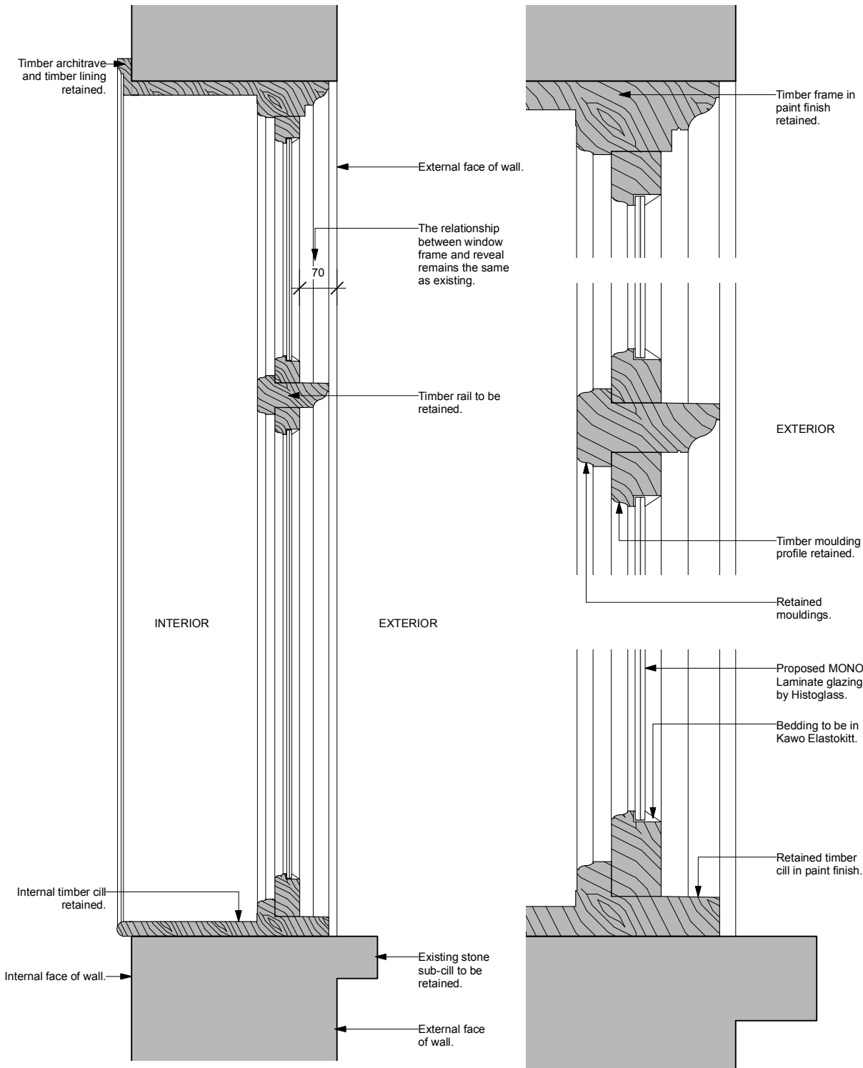
1 PROPOSED SECTION Scale 1:10 @ A3
