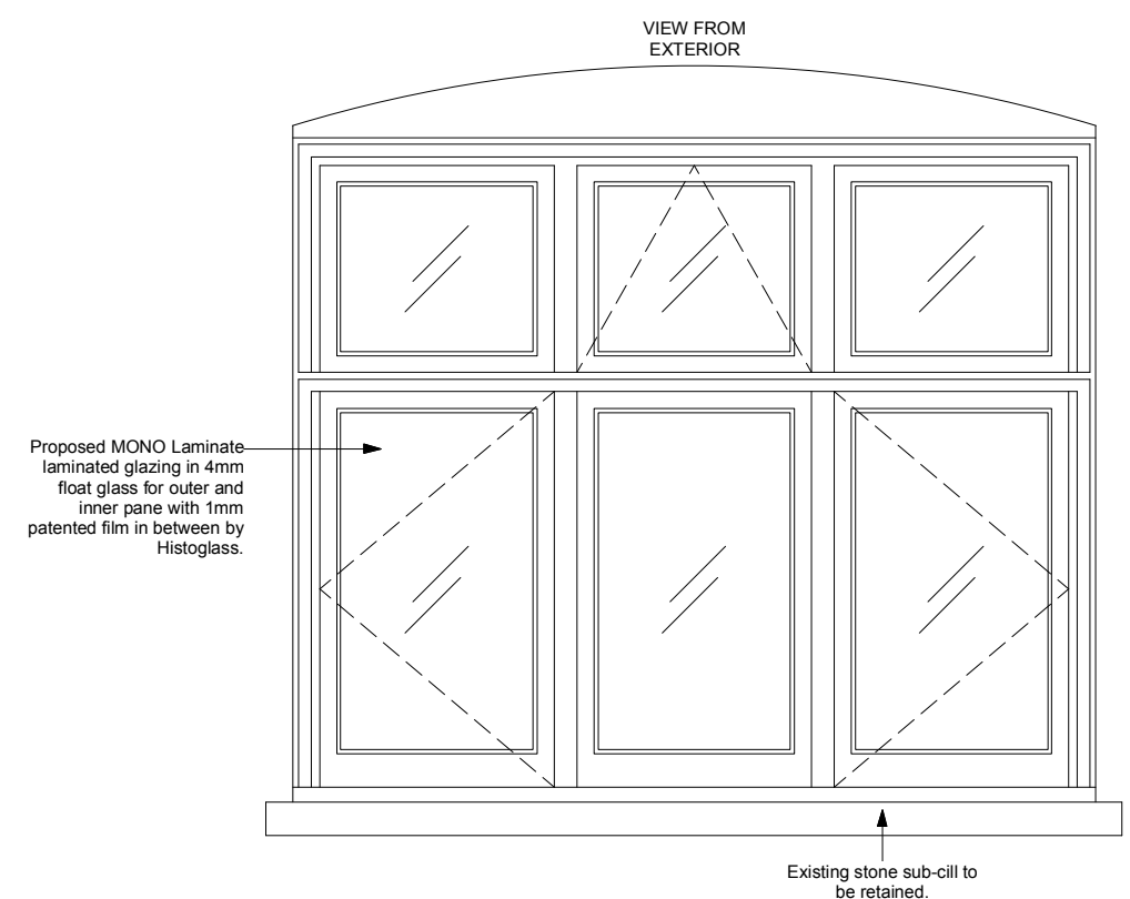
3 PROPOSED ELEVATION Scale 1:10 @ A3
