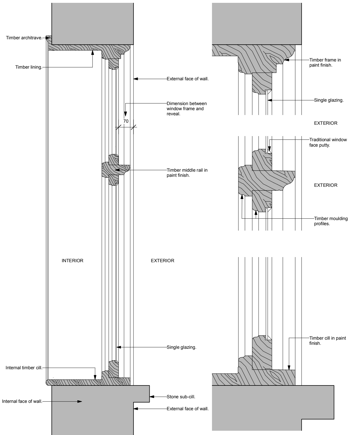
1 EXISTING SECTION Scale 1:10 @ A3
