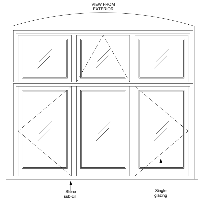
3 EXISTING ELEVATION Scale 1:10 @ A3
