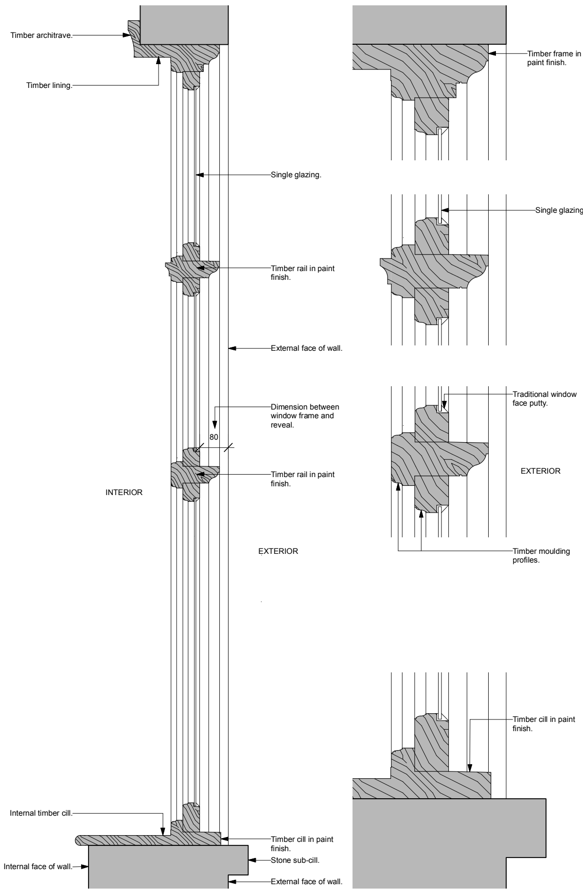
1 EXISTING SECTION Scale 1:10 @ A3
