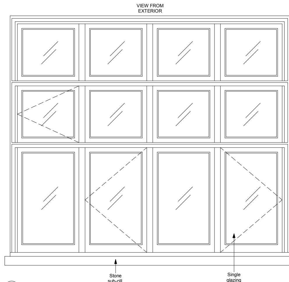
3 EXISTING ELEVATION Scale 1:20 @ A3
