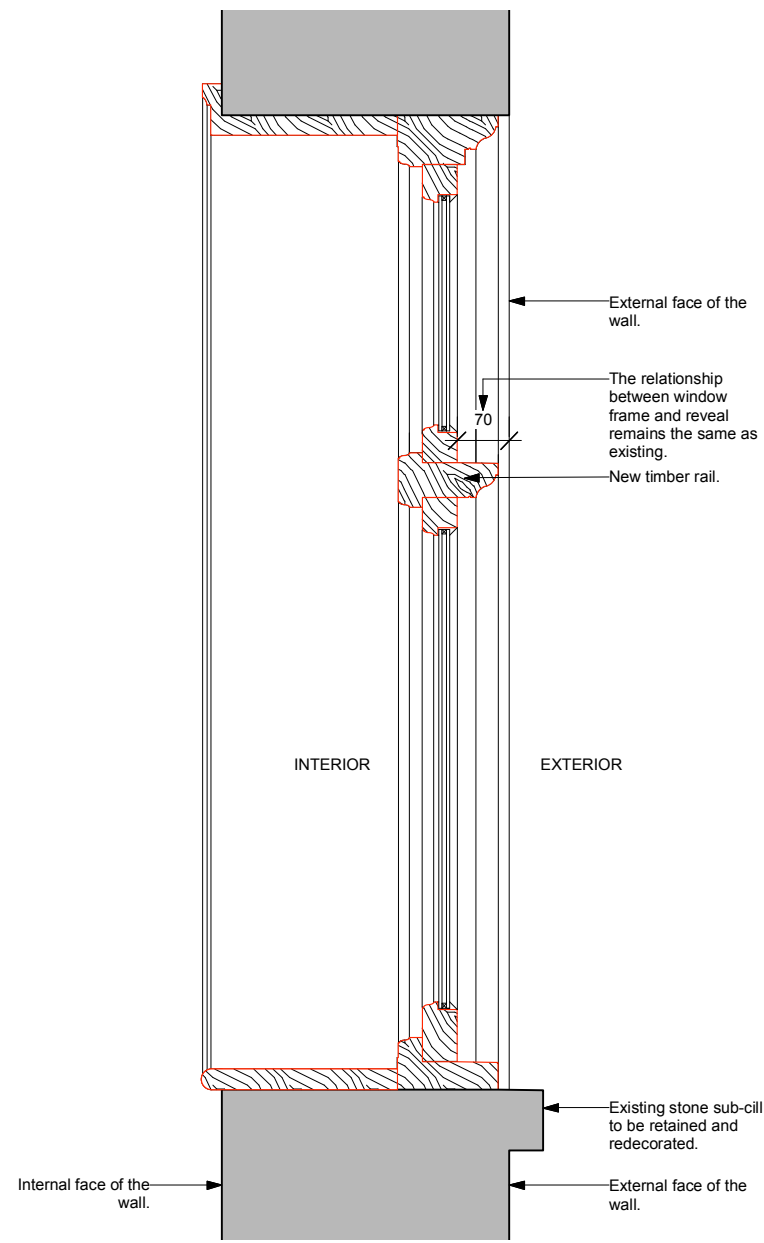
1 PROPOSED SECTION Scale 1:10 @ A3
