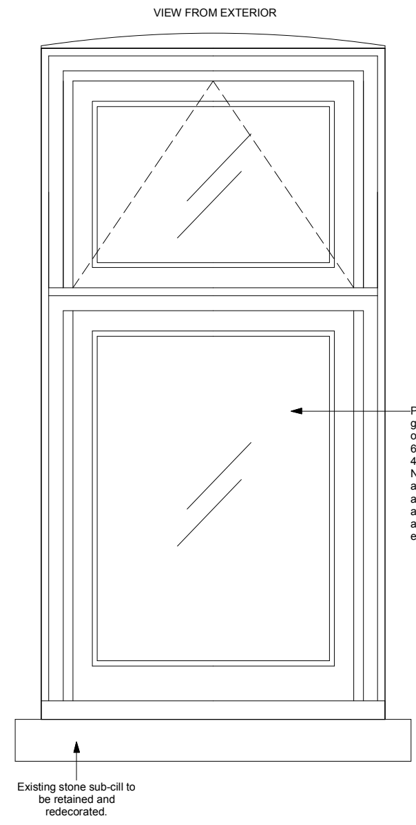
3 PROPOSED ELEVATION Scale 1:10 @ A3
