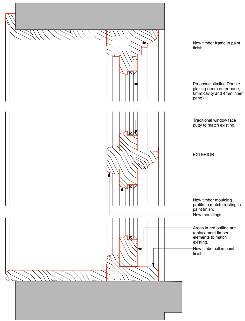
2 PROPOSED DETAILED SECTION Scale 1:5 @ A3
