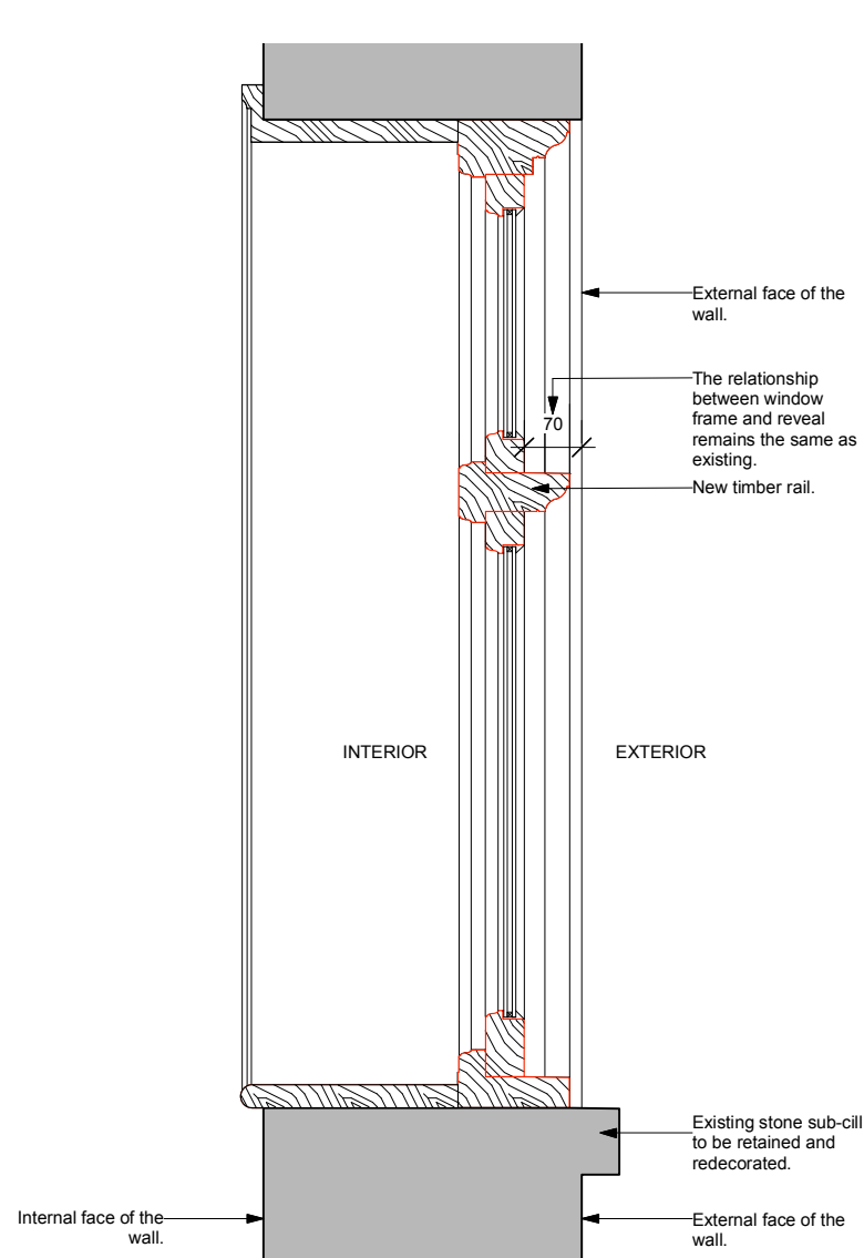
1 PROPOSED SECTION Scale 1:10 @ A3
