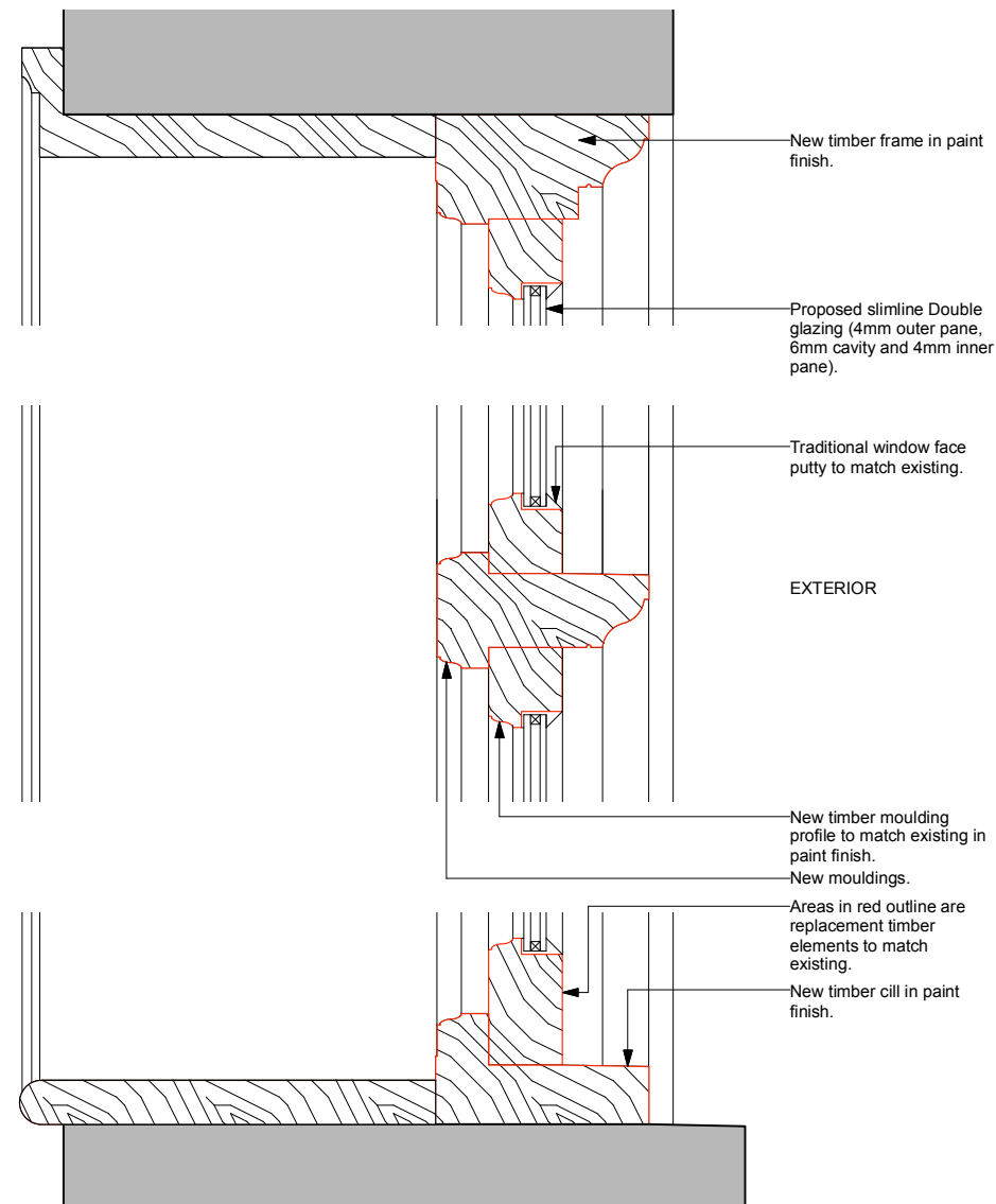
2 PROPOSED DETAILED SECTION Scale 1:5 @ A3
