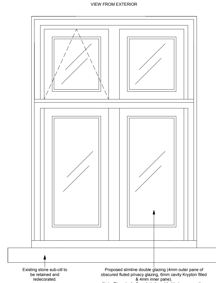
3 PROPOSED ELEVATION Scale 1:10 @ A3
