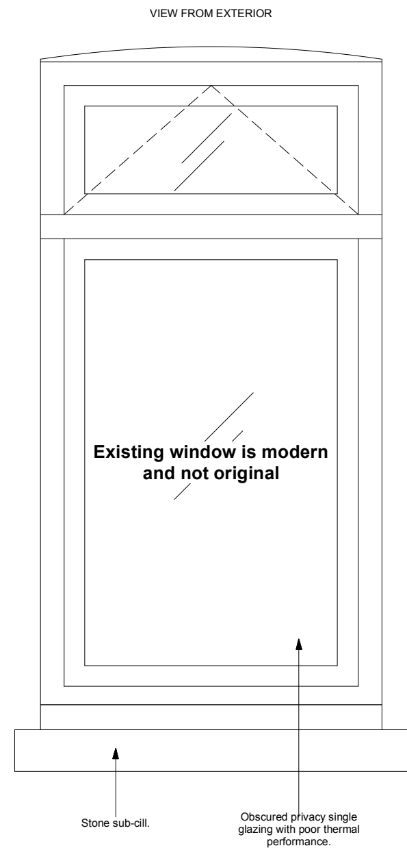
3 EXISTING ELEVATION Scale 1:10 @ A3
