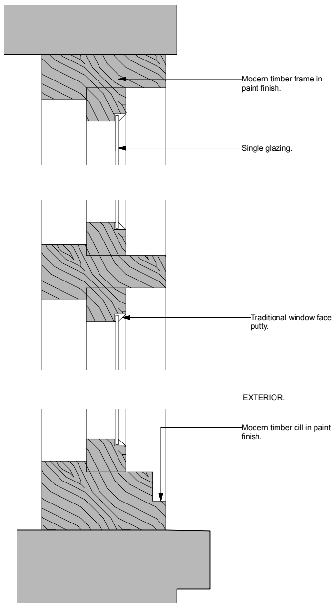
2 EXISTING DETAILED SECTION Scale 1:5 @ A3
