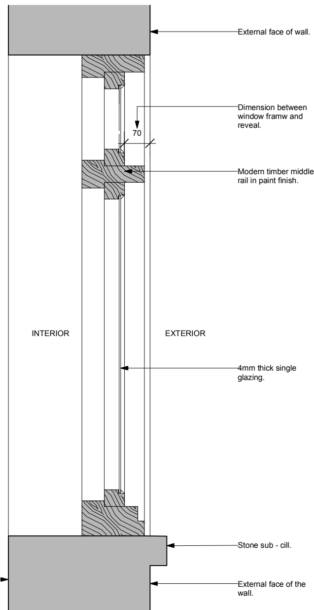
1 EXISTING SECTION Scale 1:10 @ A3
