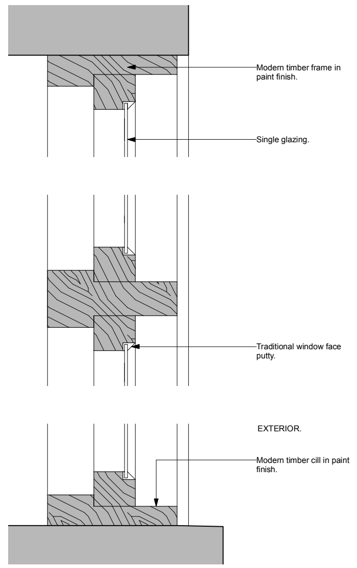
2 EXISTING DETAILED SECTION Scale 1:5 @ A3
