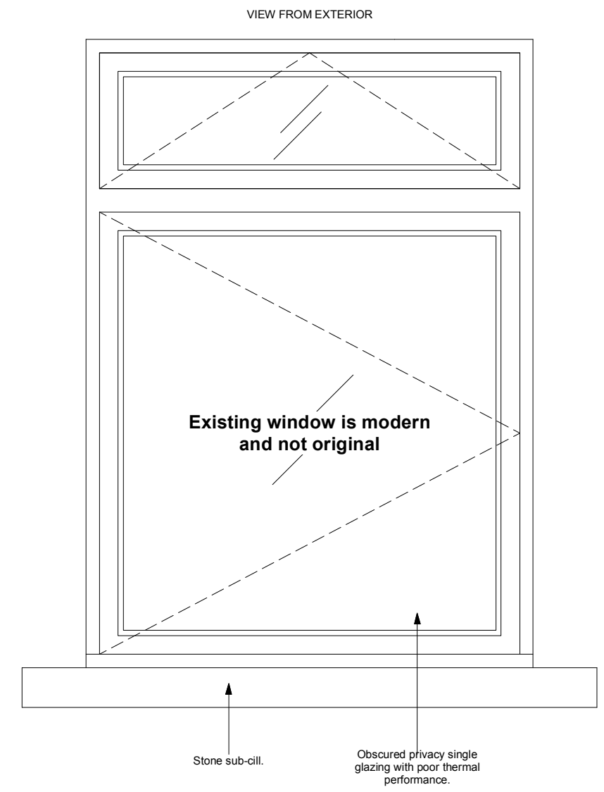
3 EXISTING ELEVATION Scale 1:10 @ A3
