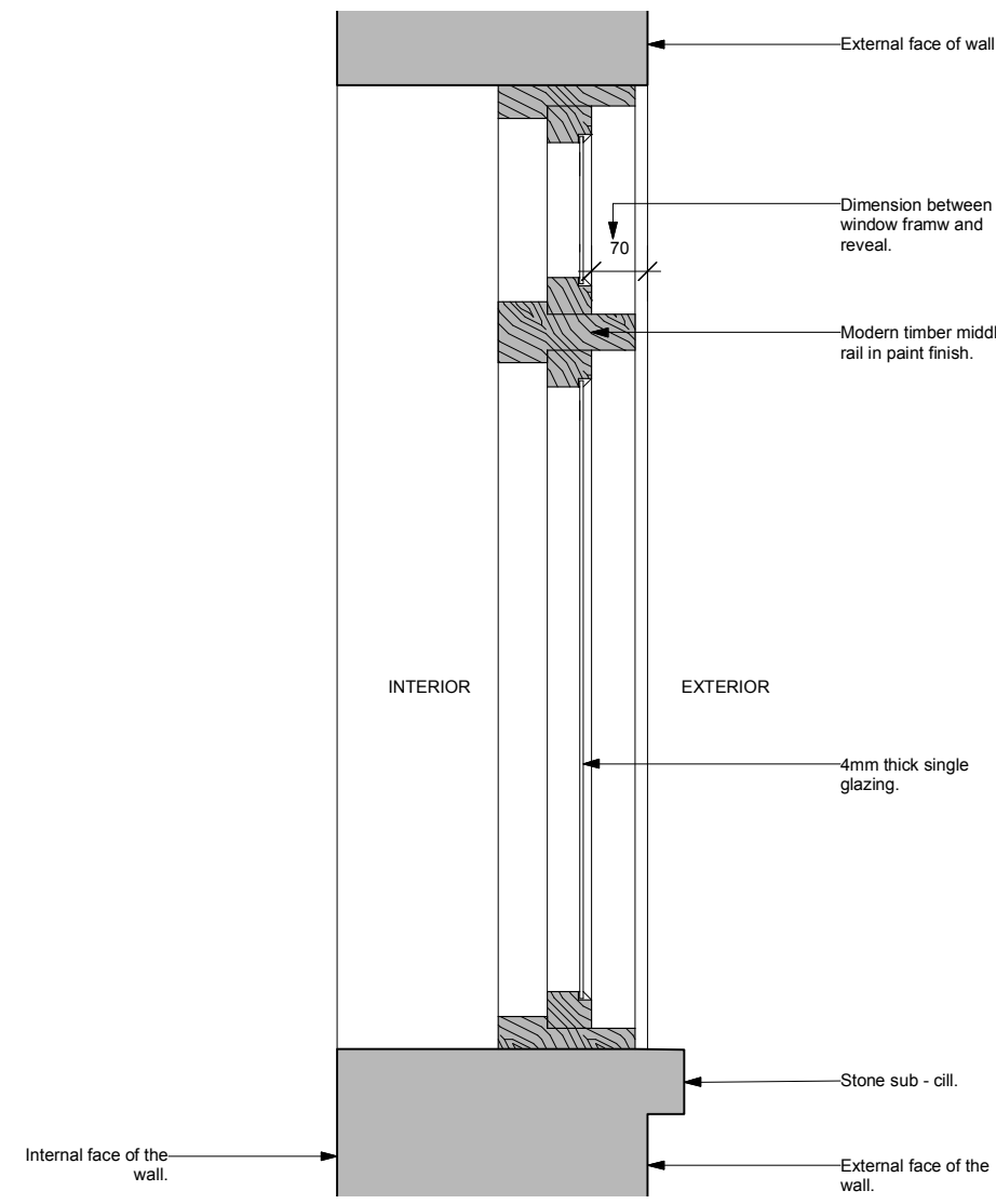
1 EXISTING SECTION Scale 1:10 @ A3
