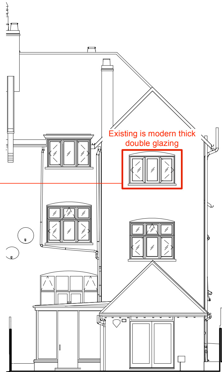
1 EXISTING REAR ELEVATION Scale 1:100 @ A3
