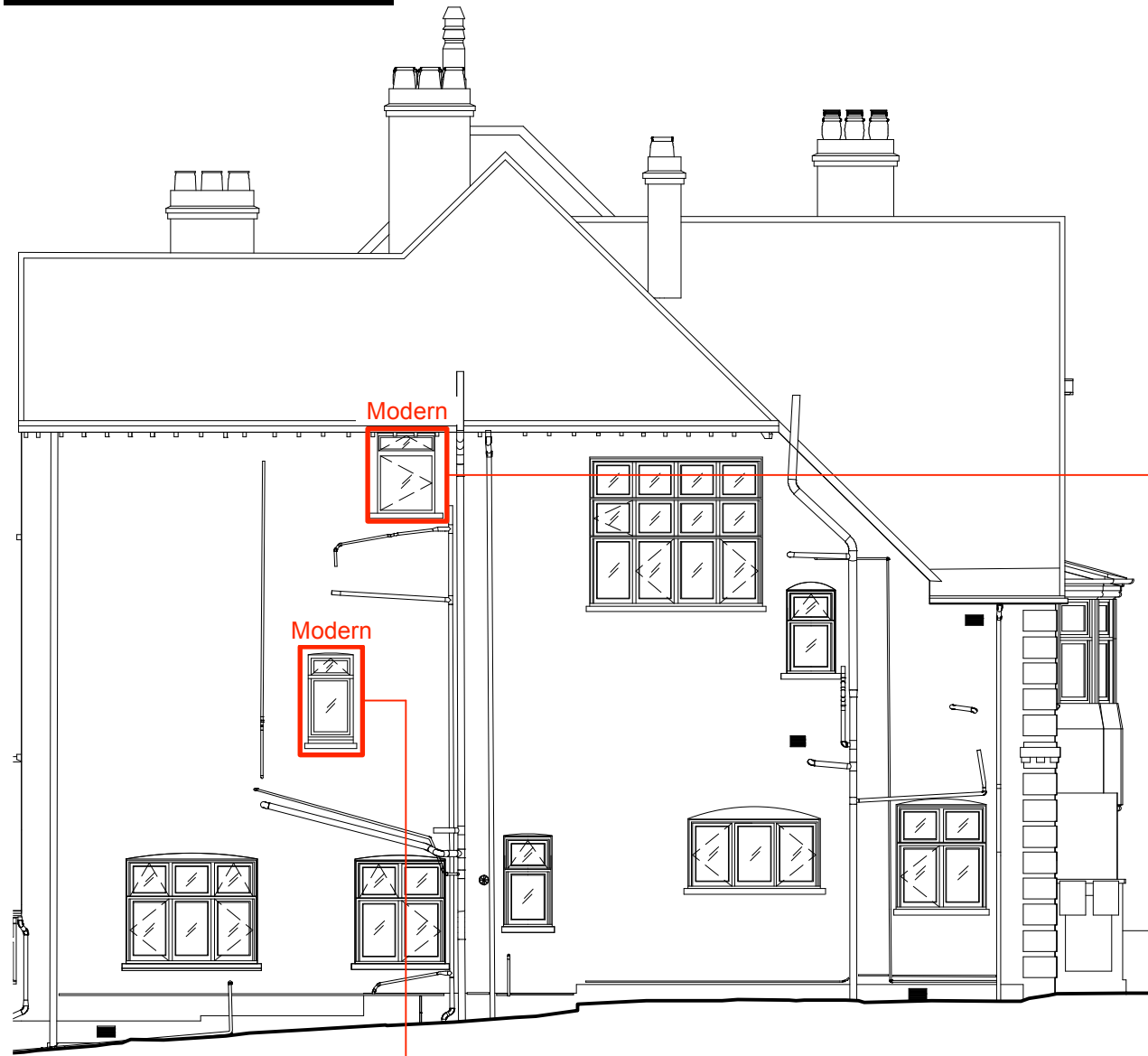
2 EXISTING SIDE ELEVATION Scale 1:100 @ A3
