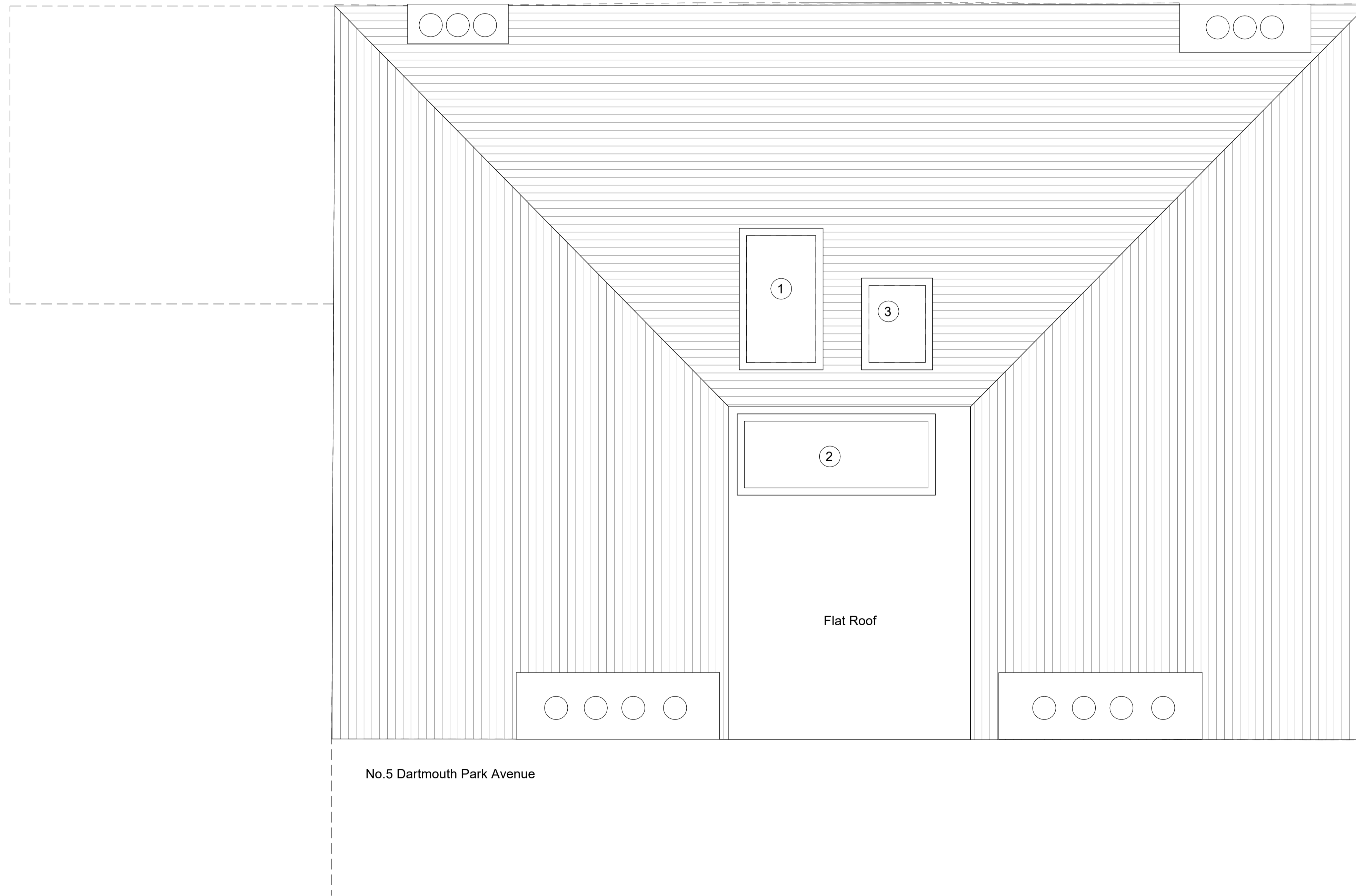
1 Proposed Roof Plan 1:25
