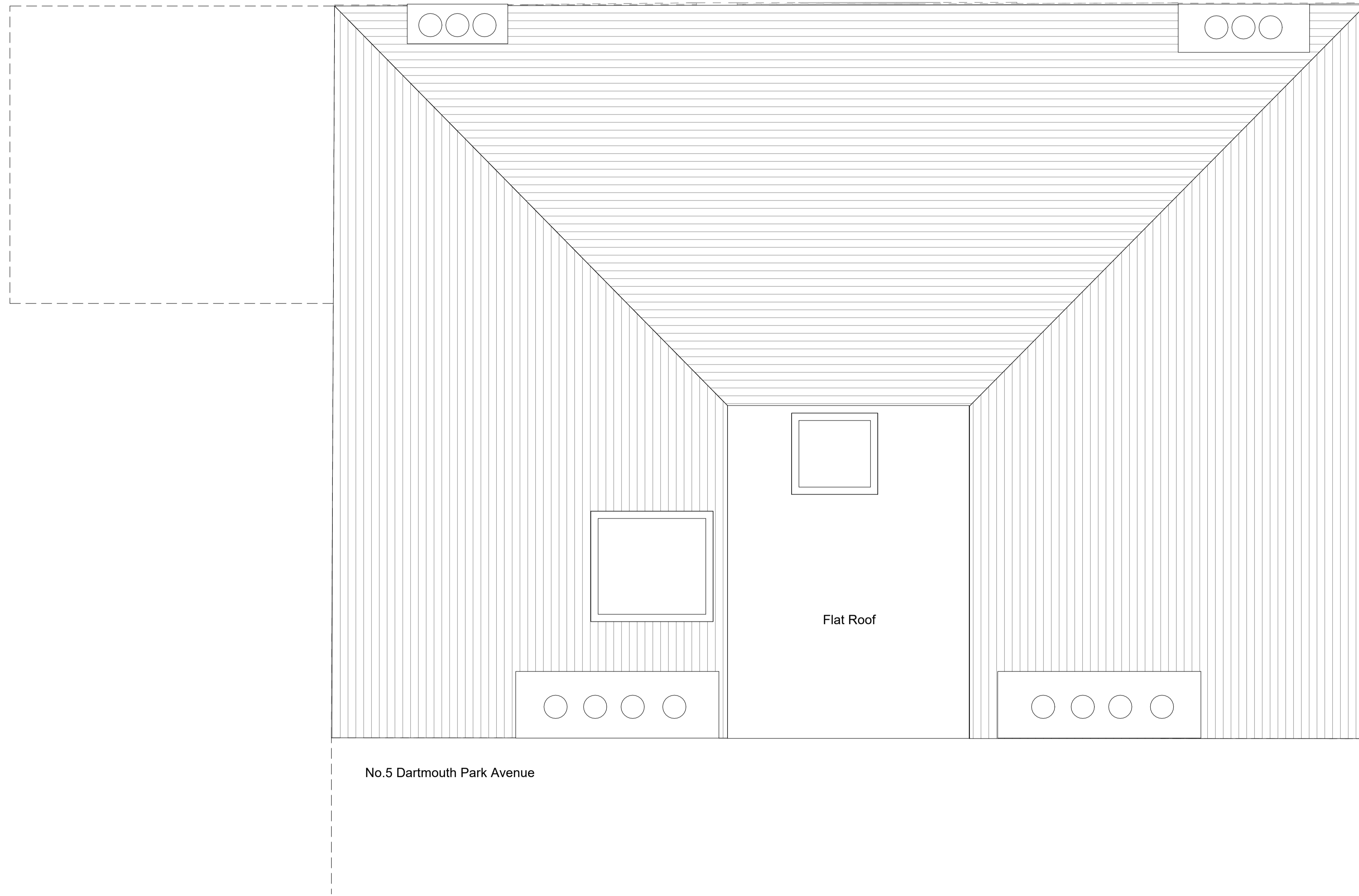
1 Existing Roof Plan 1:25
