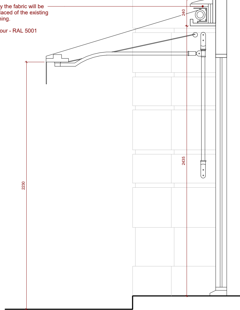
SECTION - AWNING OPEN
