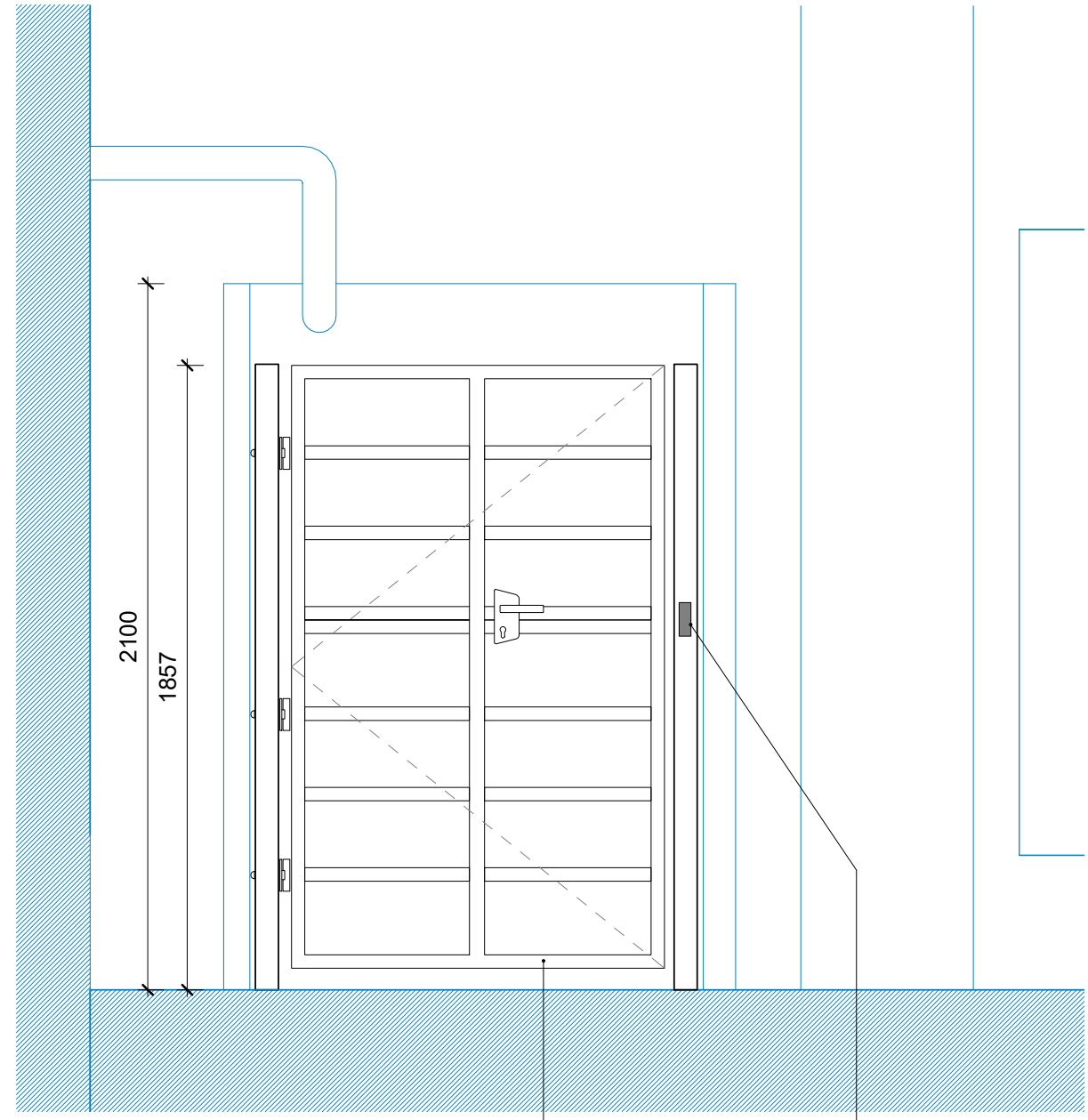
2 ELEVATION - Escape Gate 1 : 20
