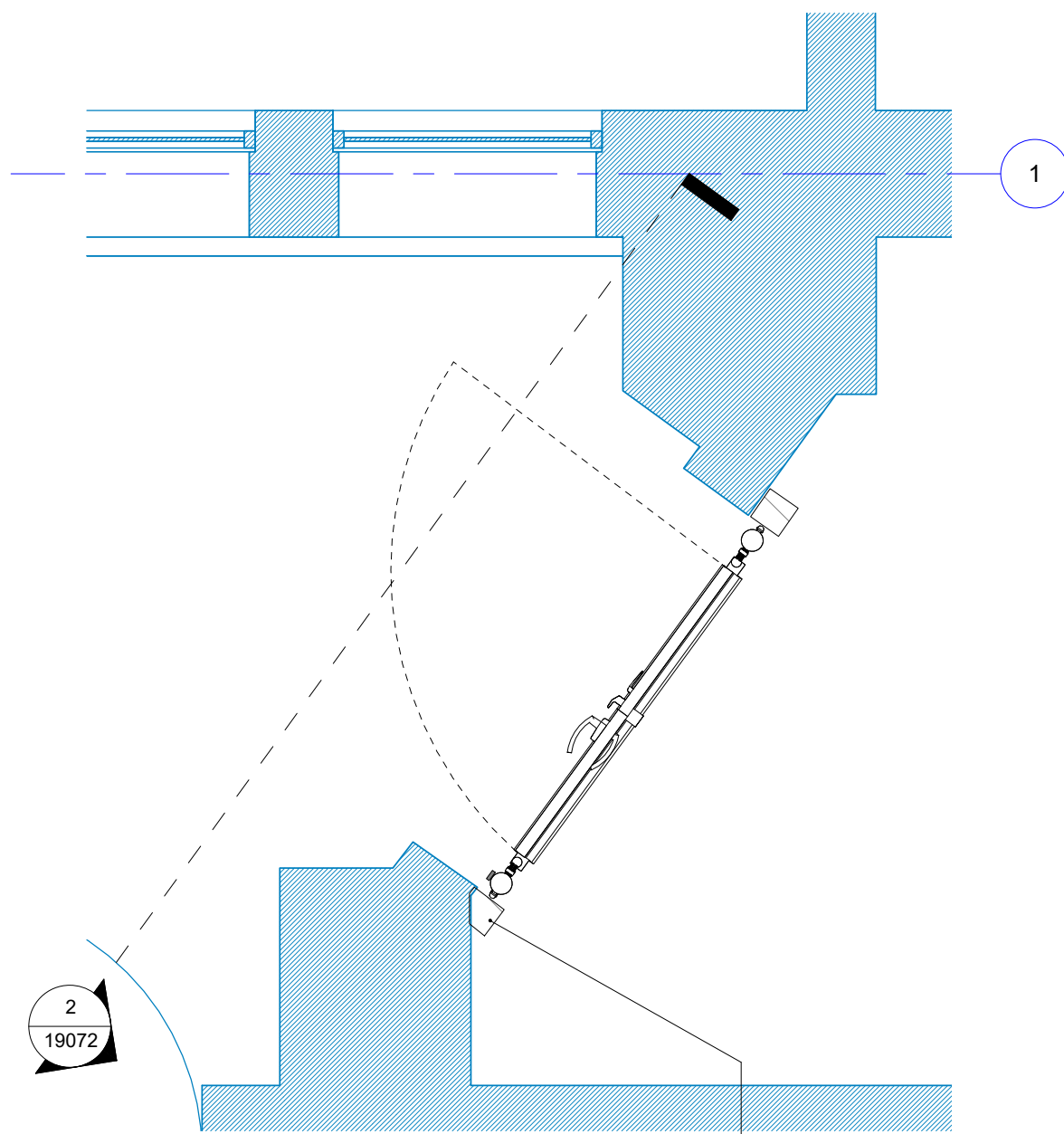
1 Proposed LG - Gower Street Escape Gate 1 : 20
