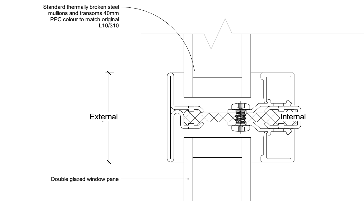
6 W-LG26 Detail Transom 1 : 2
