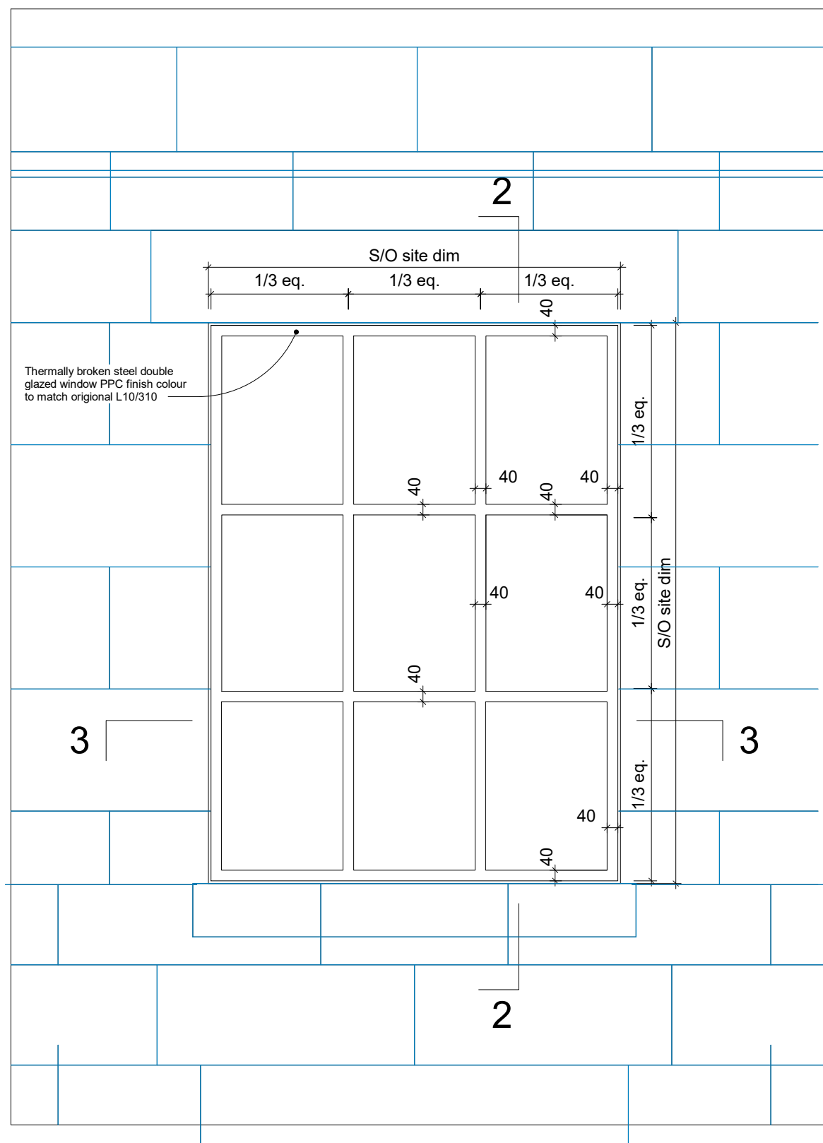
3 W-LG26 Detail Front 1 : 20
