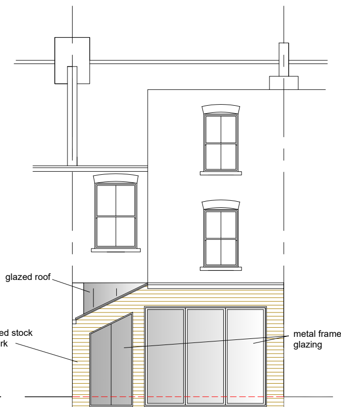
REAR ELEVATION
