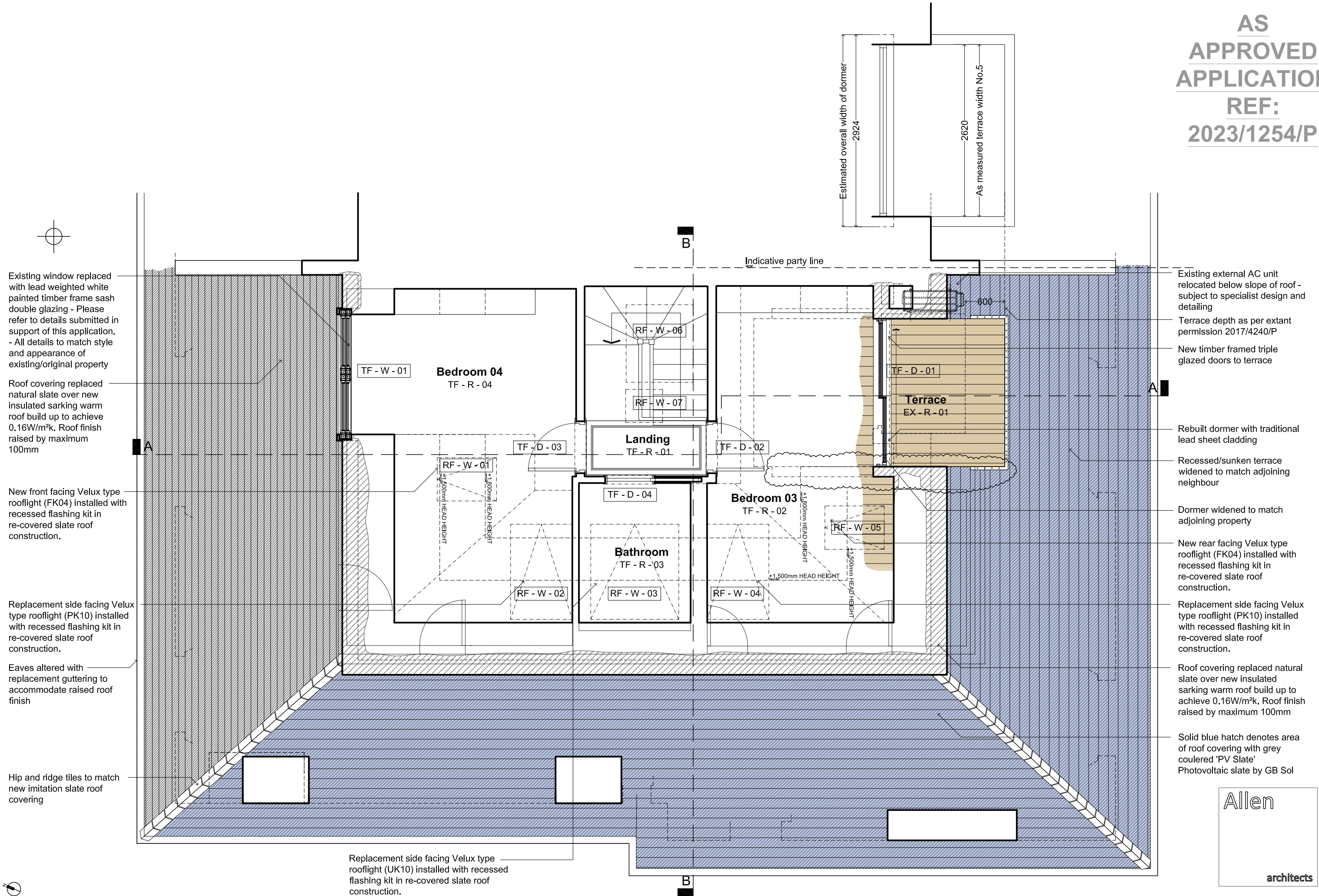
PROPOSED THIRD FLOOR PLAN SCALE 1:50
