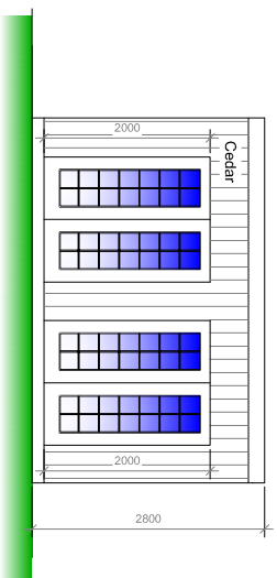
FRONT ELEVATION
