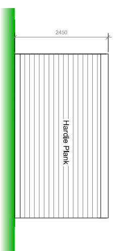
REAR ELEVATION
