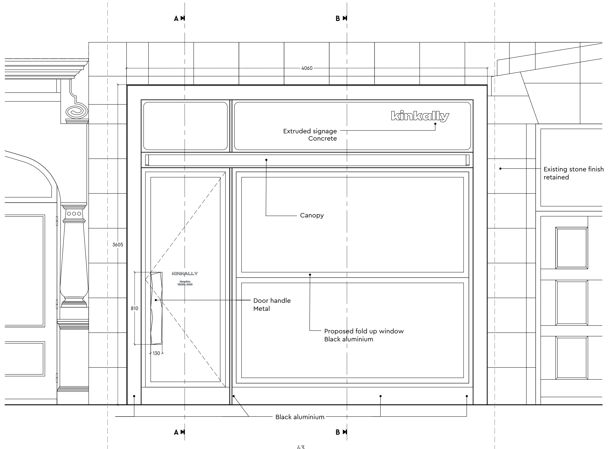
Proposed facade elevation (detail) M 1:20
