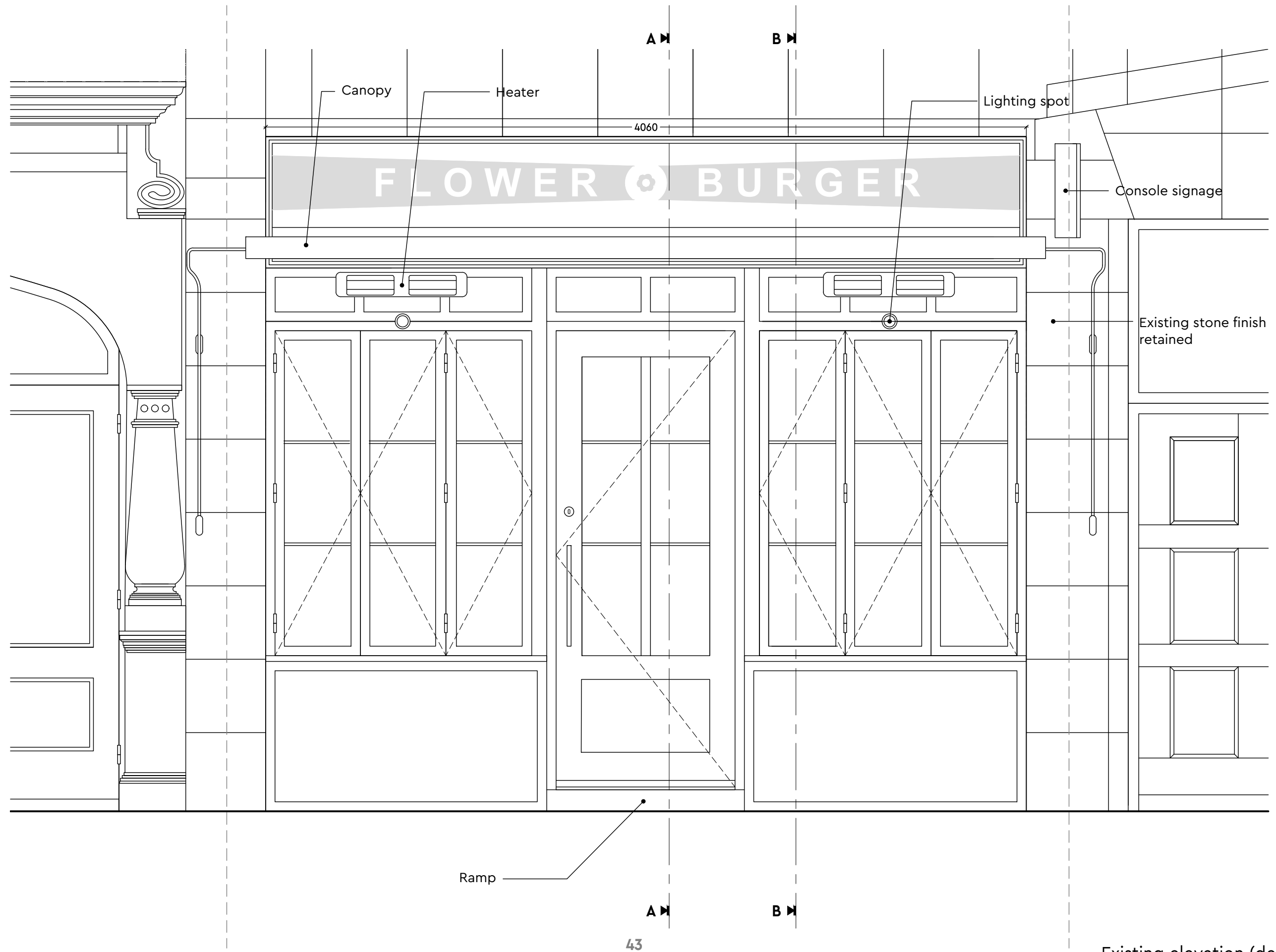
Existing elevation (detail) M 1:20
