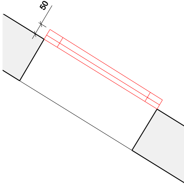
01 Existing Rooflights
