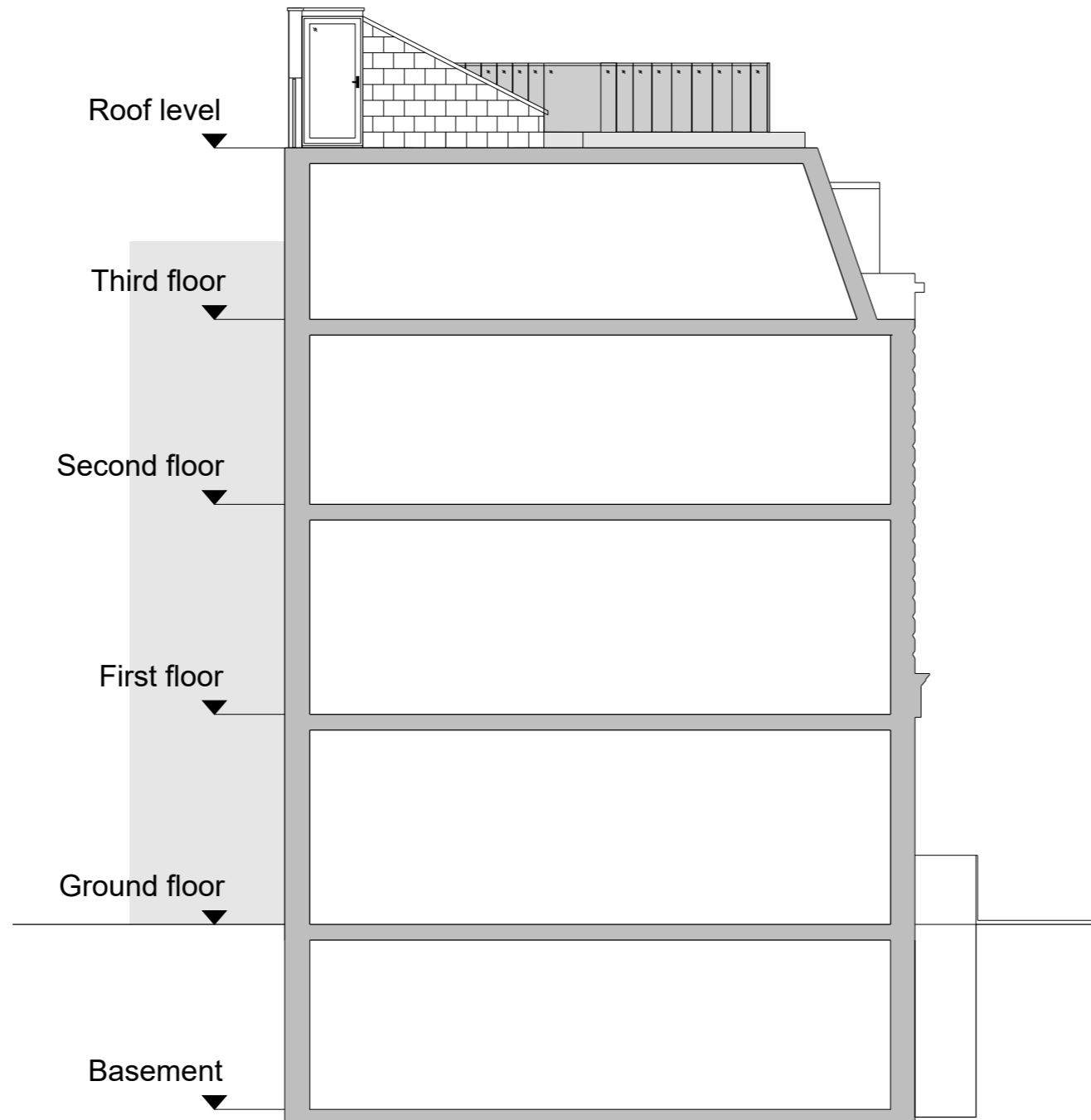
Proposed section 1-1
