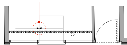
01 PROPOSED SHOP FRONT | SHOWING GRILLS CLOSED GA PLAN 1:50
