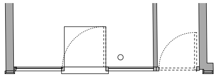
01 EXISTING SHOP FRONT GA PLAN 1:50
