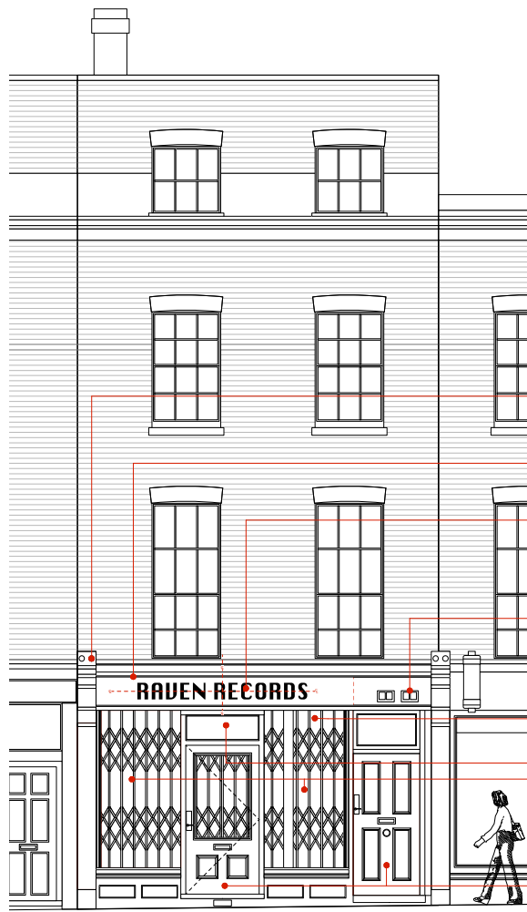
02 PROPOSED SHOP FRONT | SHOWING GRILLS CLOSED FRONT ELEVATION 1:50
