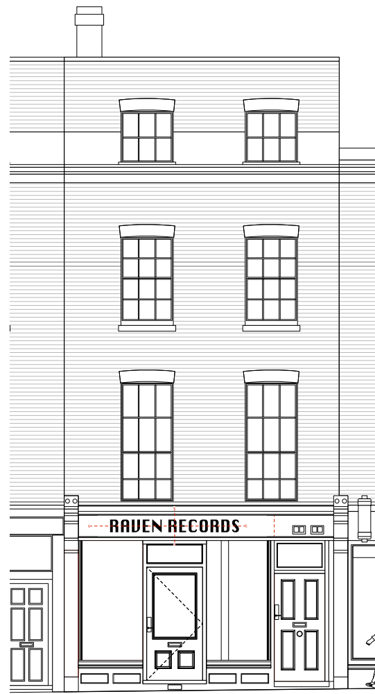
02 PROPOSED SHOP FRONT | SHOWING GRILLS OPEN FRONT ELEVATION 1:50
