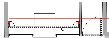
01 PROPOSED SHOP FRONT | SHOWING GRILLS OPEN GA PLAN 1:50
