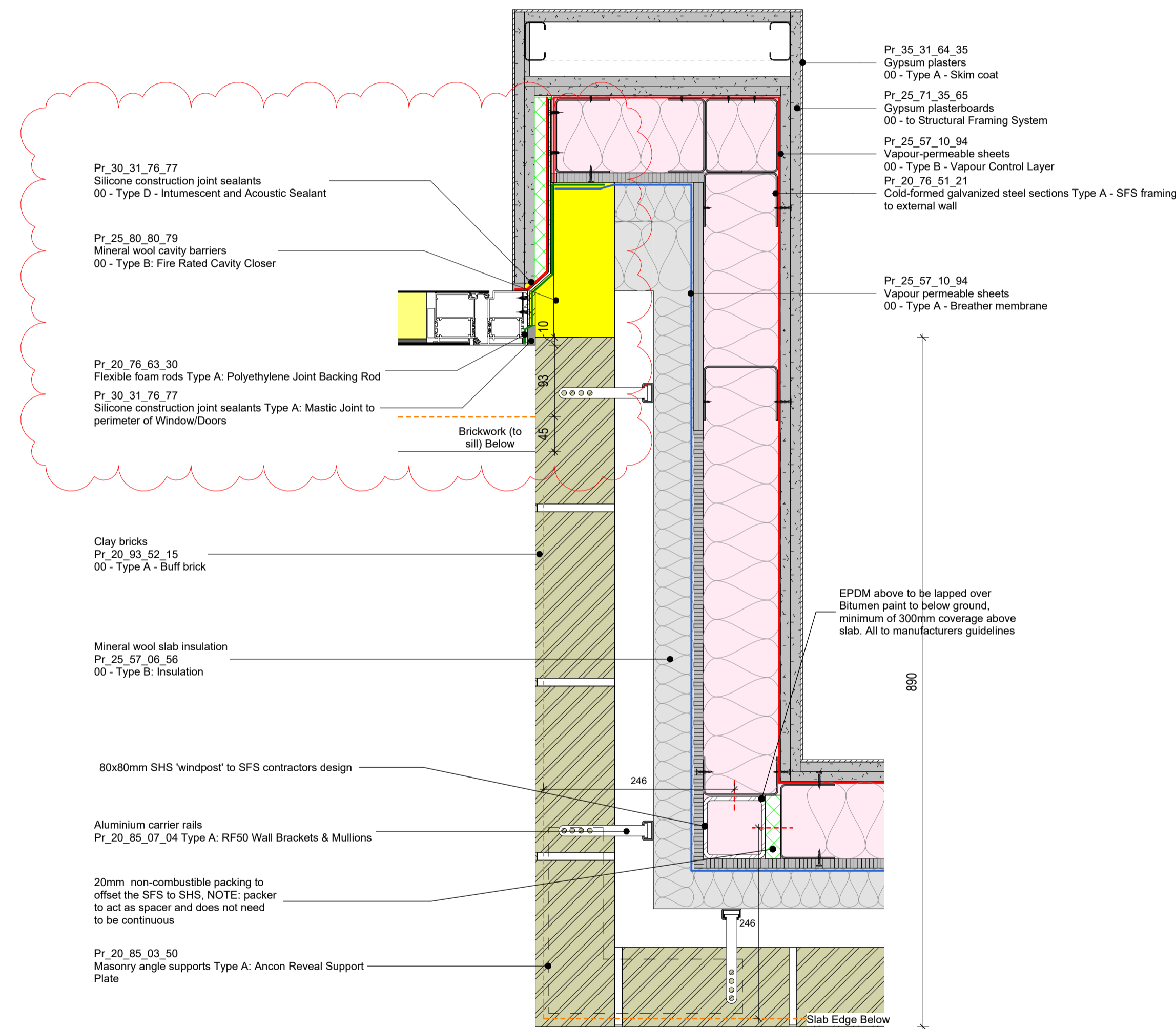
2 Plan Detail - Bay Window Corner Support - Below Window 1 : 5
