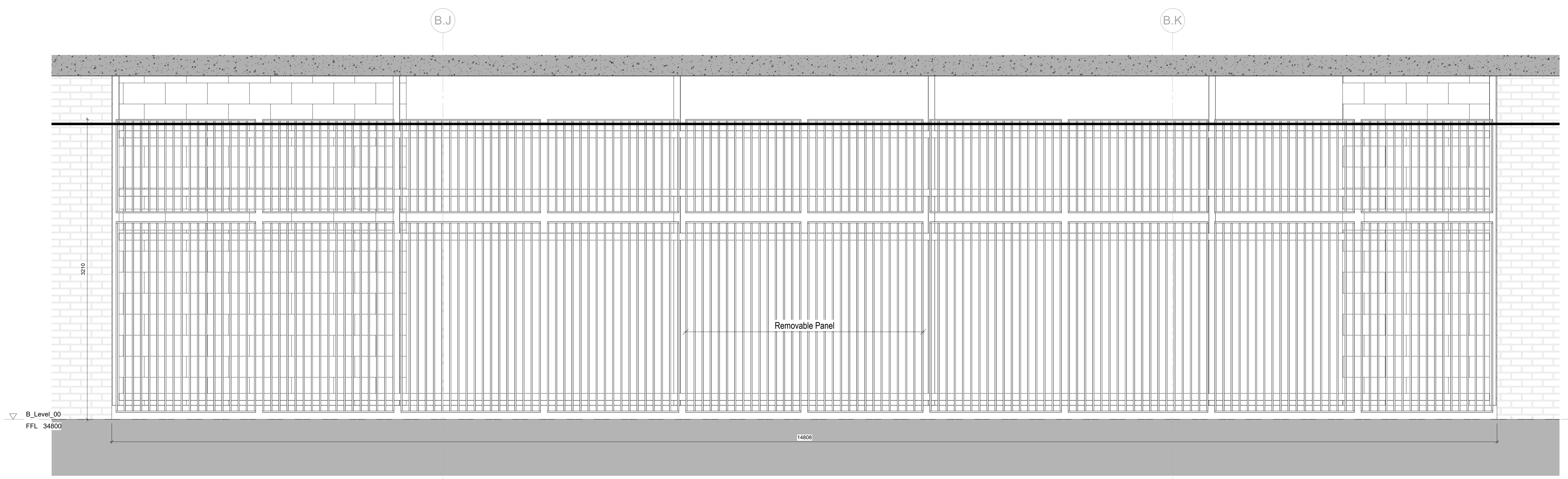
1 Cladding Bay Study 03 - Dependent 1 1:20
