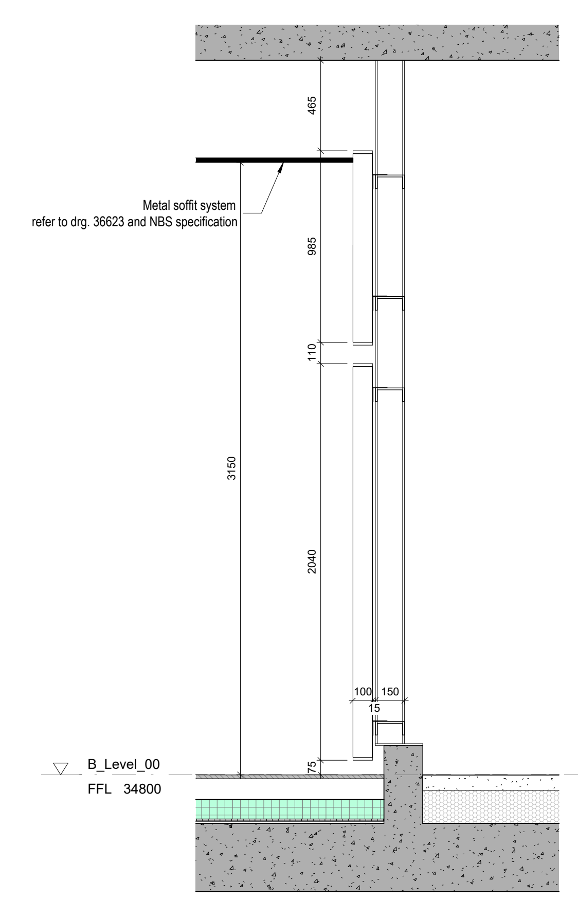
3 Cladding Bay Study 03 Section 1:20
