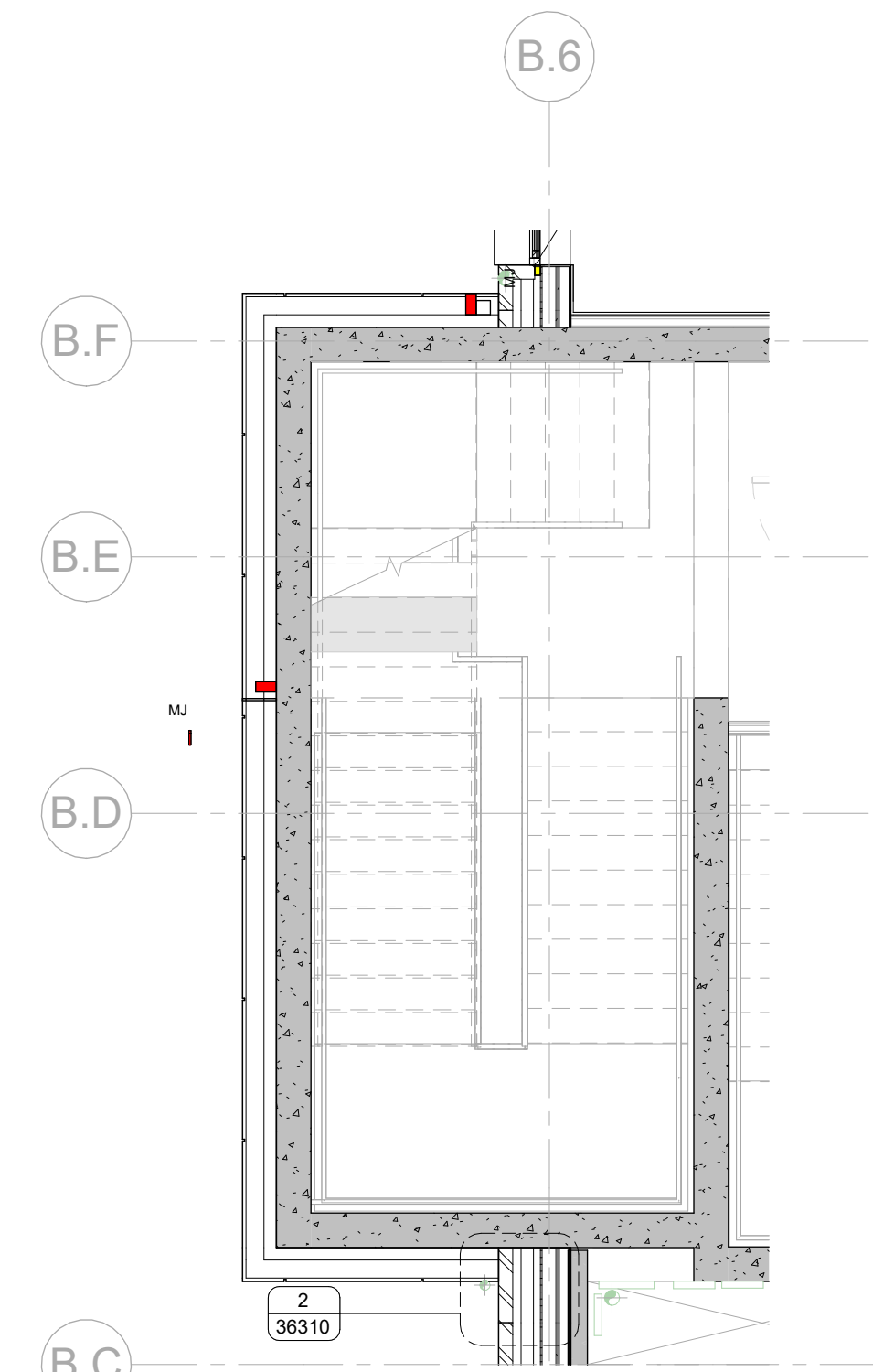
5 South Escape Staircase - Roof Level 1:50
