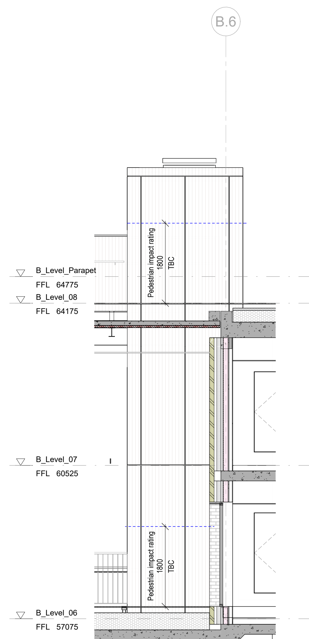
2 South Escape Staircase - View 2 1:50
