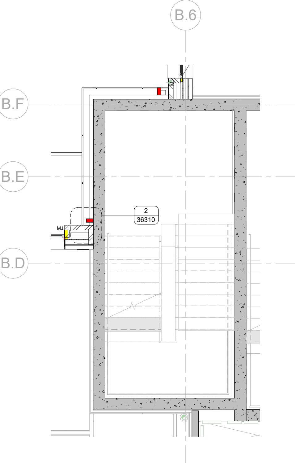
6 B_Level_05 - South Escape Stairs 1:50
