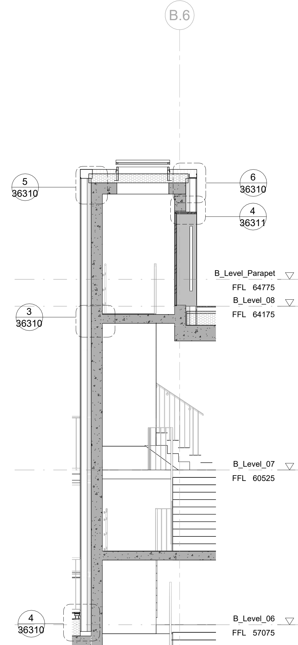
8 South Escape Staircase - Section 1:50
