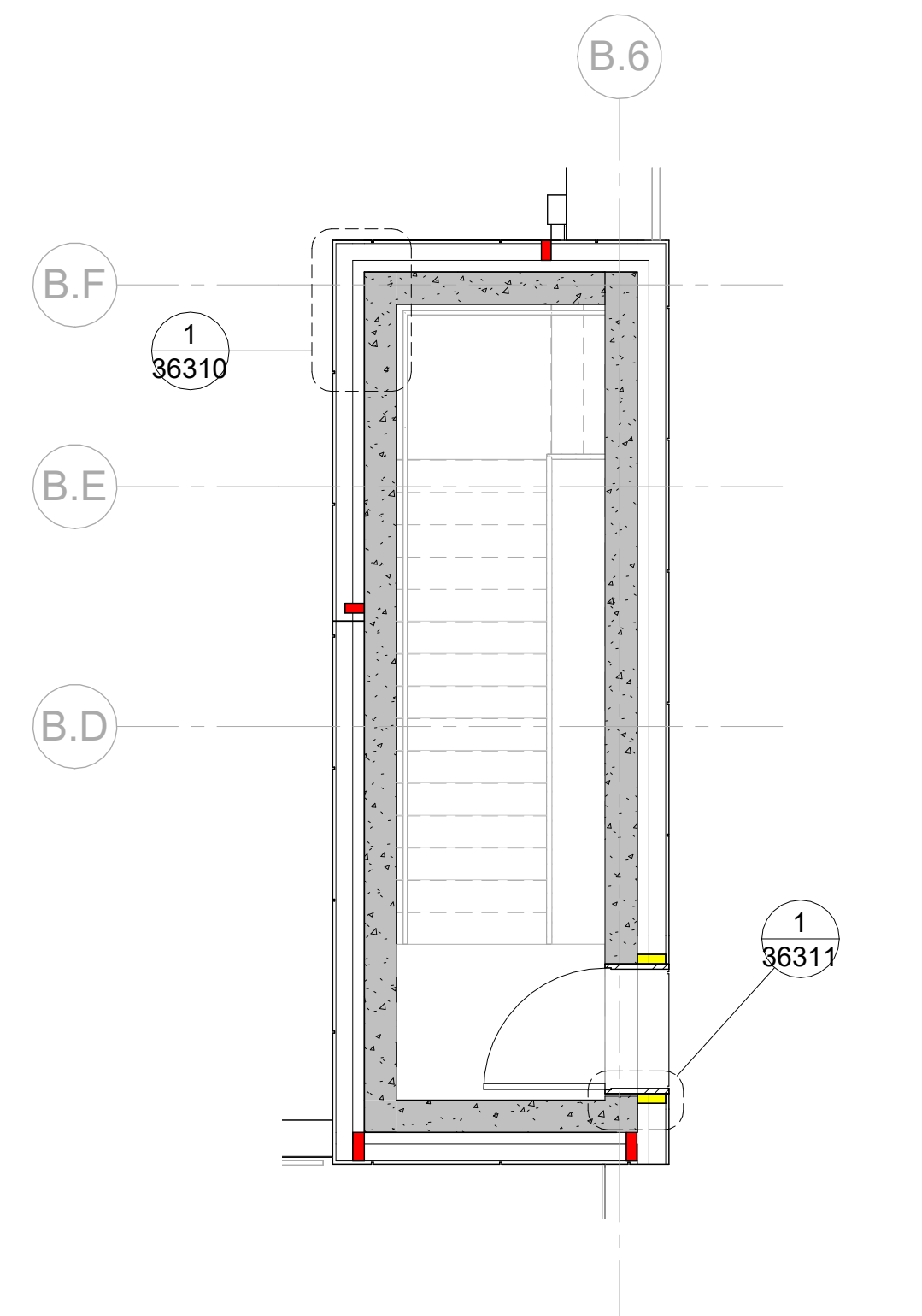
5 South Escape Staircase - Roof Level 1:50
