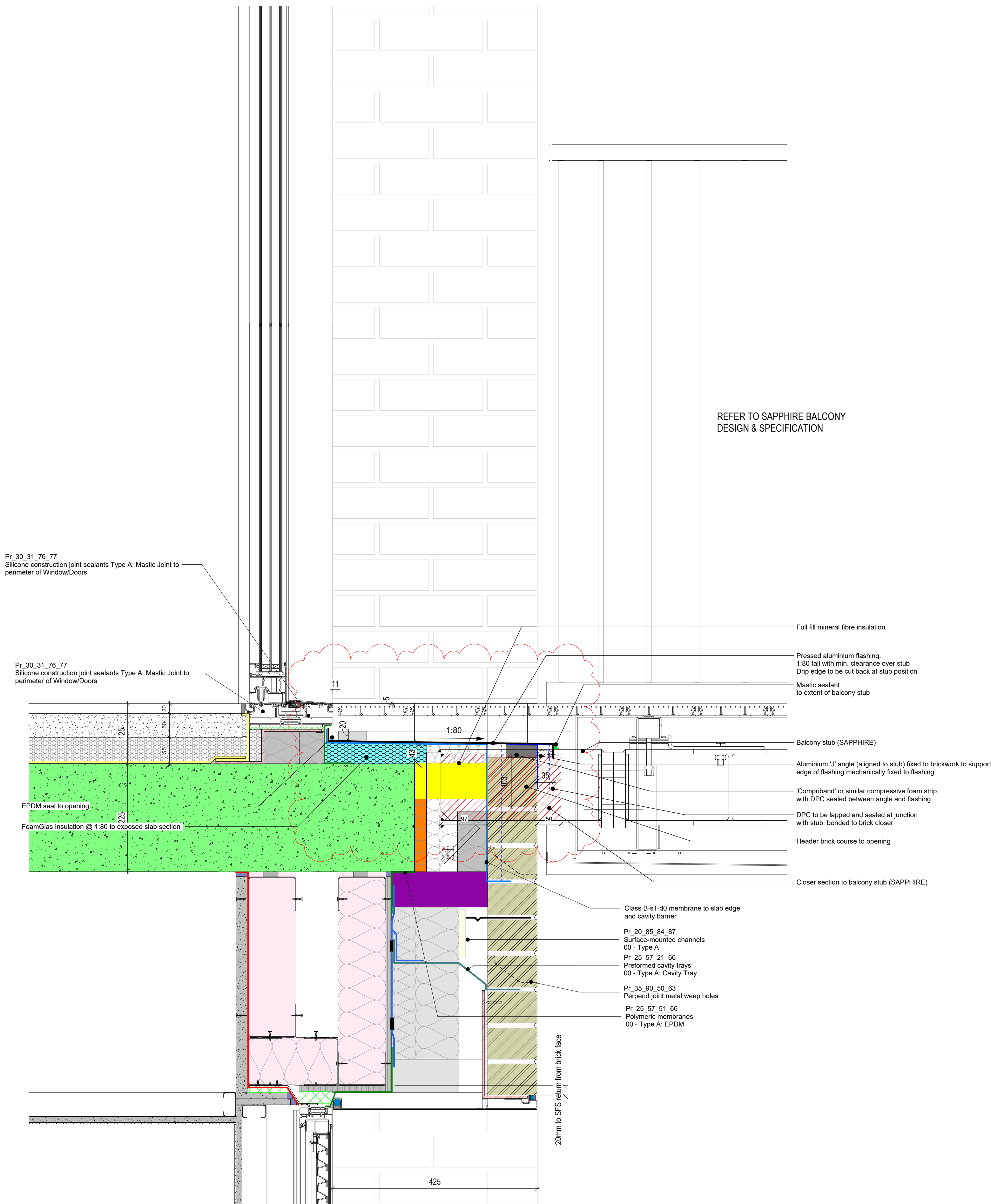
2 Balcony section detail - Flat metal front panel @ masonry support 1 : 5
