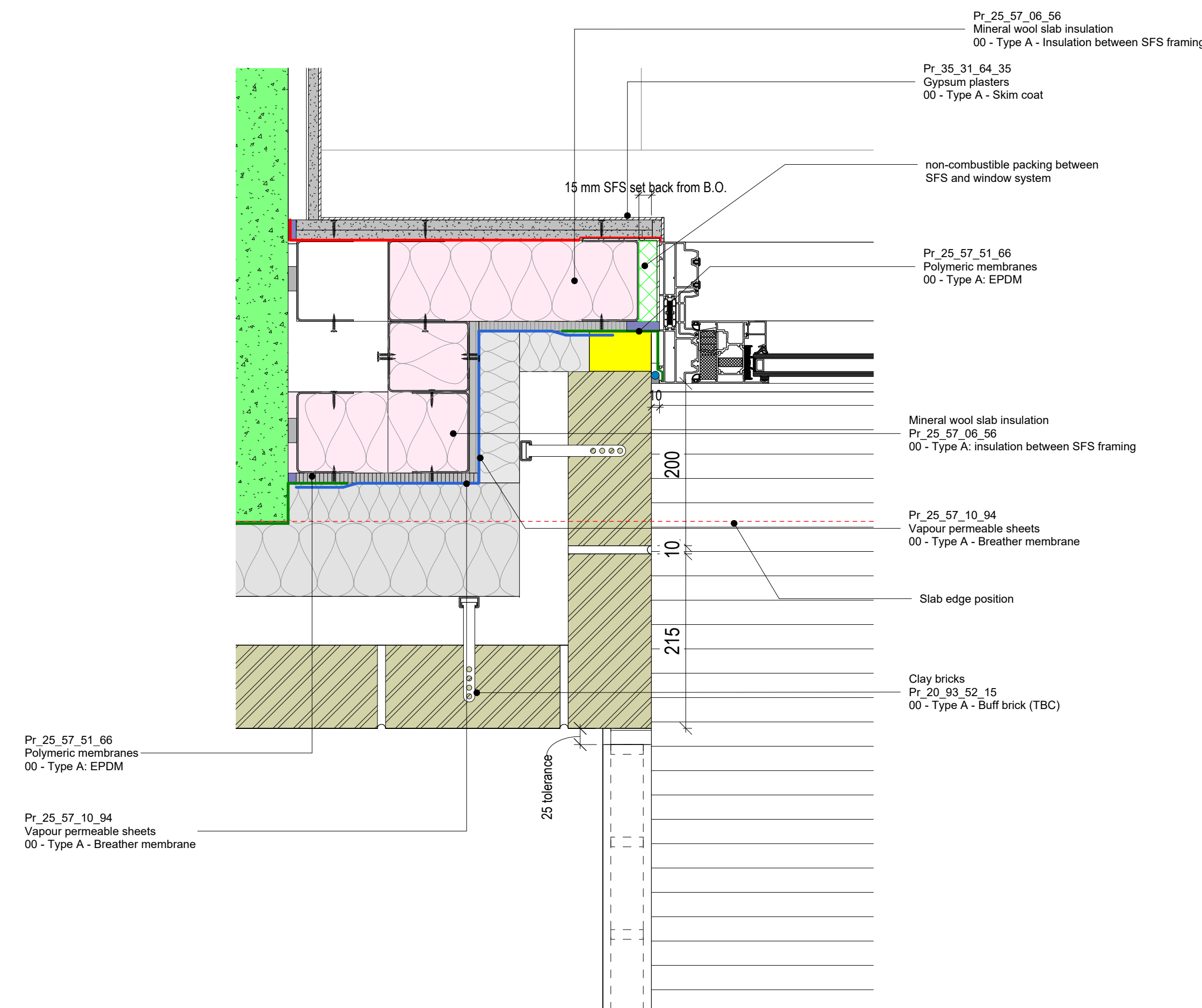
3 Flat metal front panel - Handrail jamb detail 1 : 5
