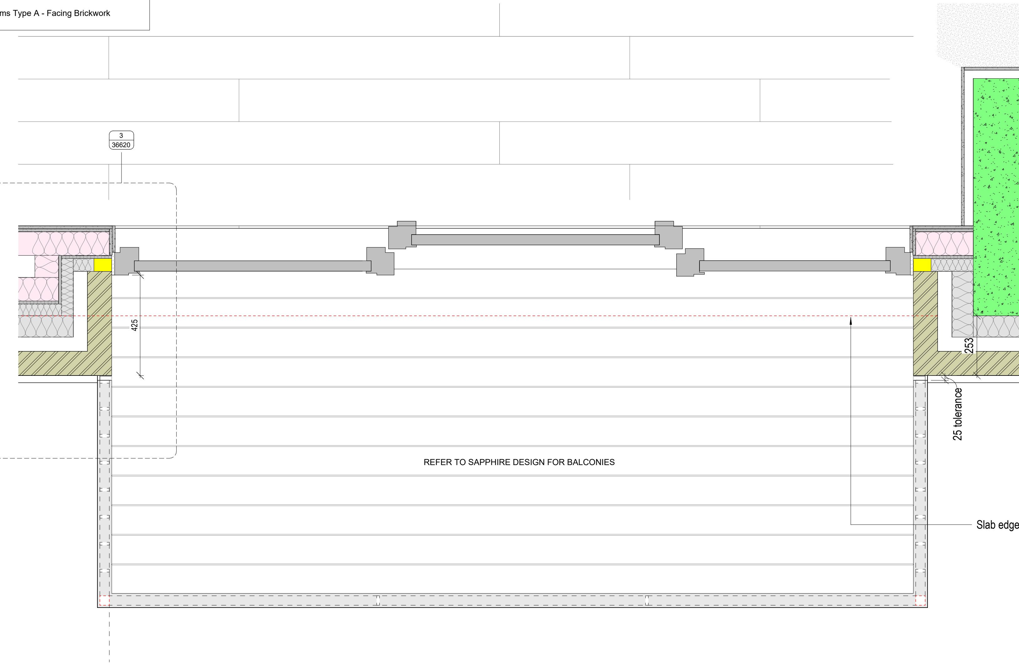
1 Balcony plan - Flat metal front panel 1 : 10
