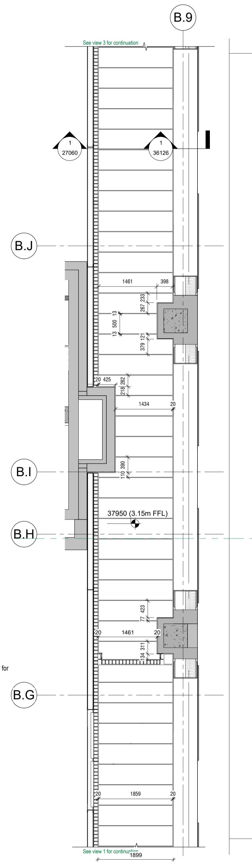
2 Building B – Level 00 – Entrance Terrace – RCP (2/3) 1 : 50
