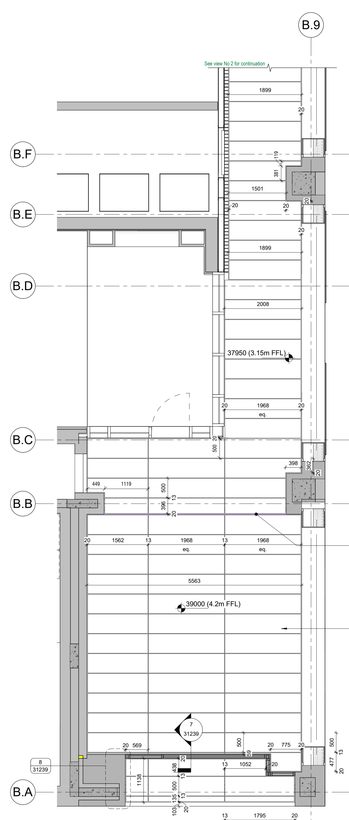
1 Building B – Level 00 – Entrance Terrace – RCP (1/3) 1 : 50
