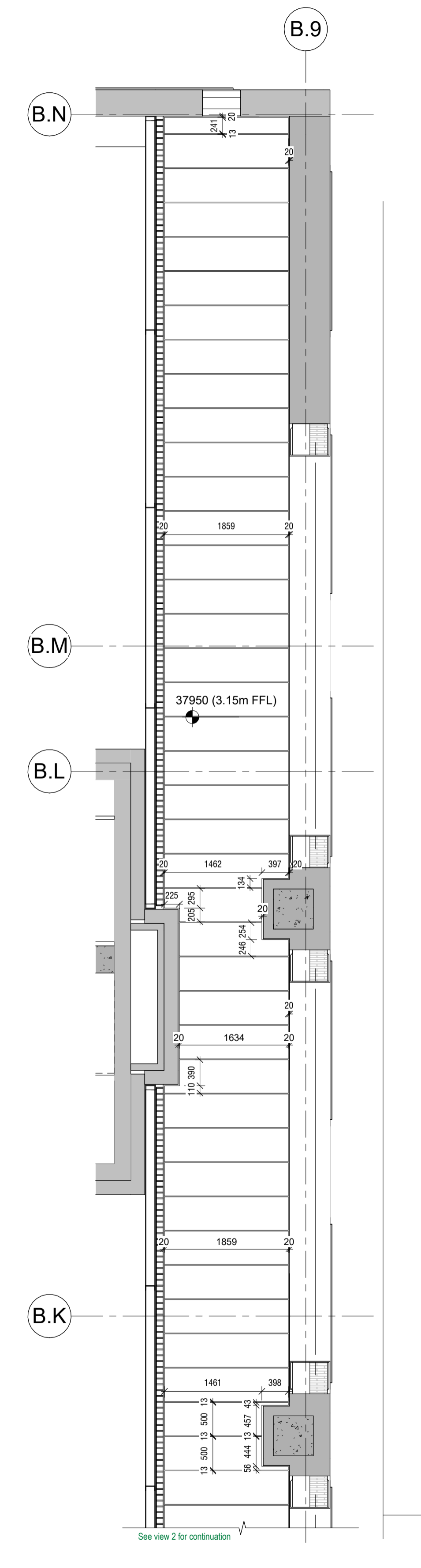
3 Building B – Level 00 – Entrance Terrace – RCP (3/3) 1 : 50
