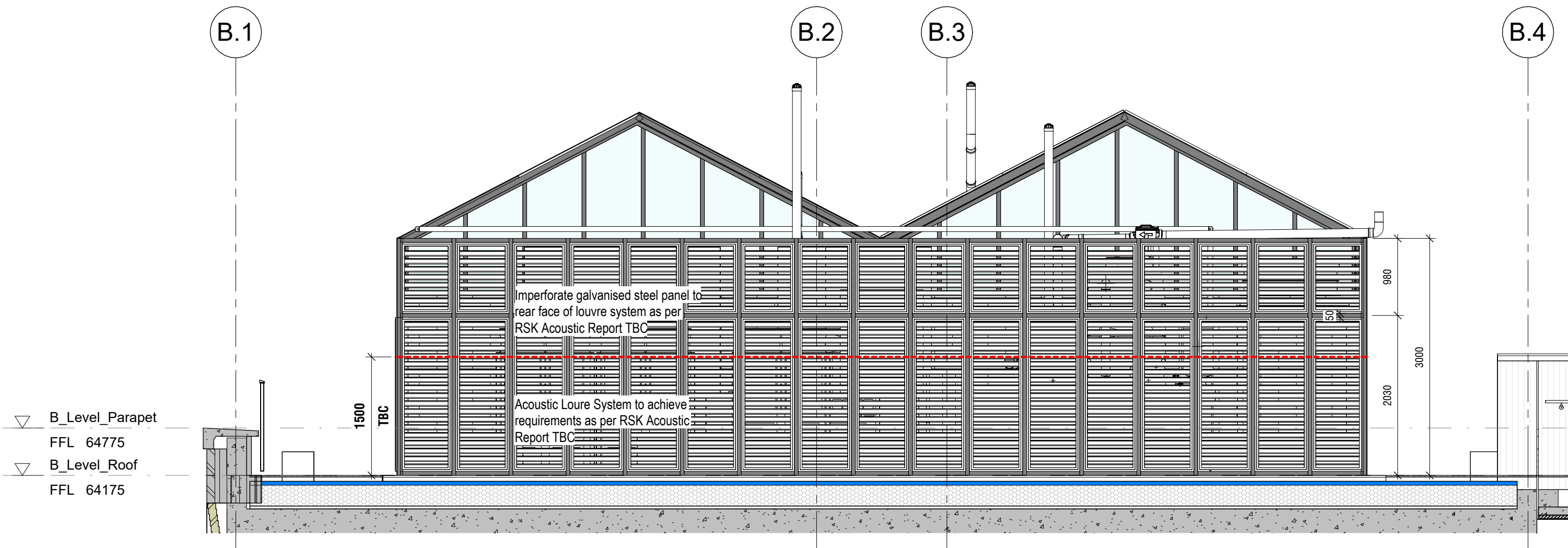
Core B3 Plantscreen - South Elevation 1 : 50
