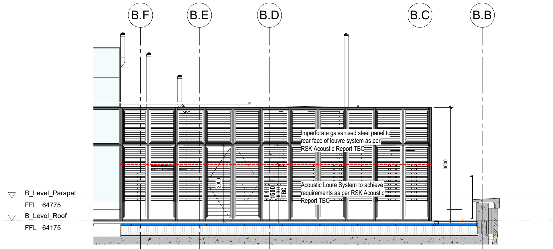
Core B3 Plantscreen - South-West Elevation 1 : 50
