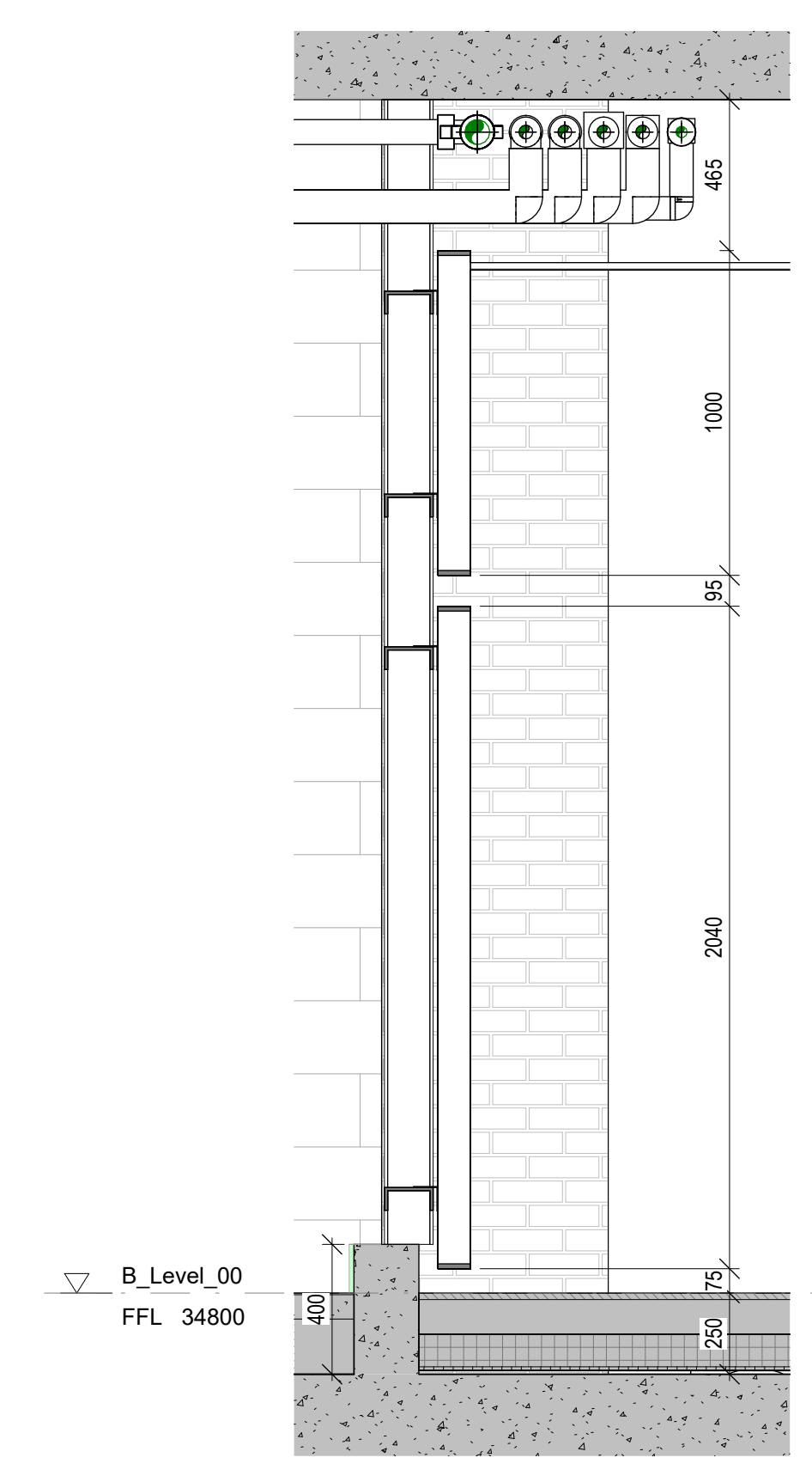
3 MWB2 - Section 1:20
