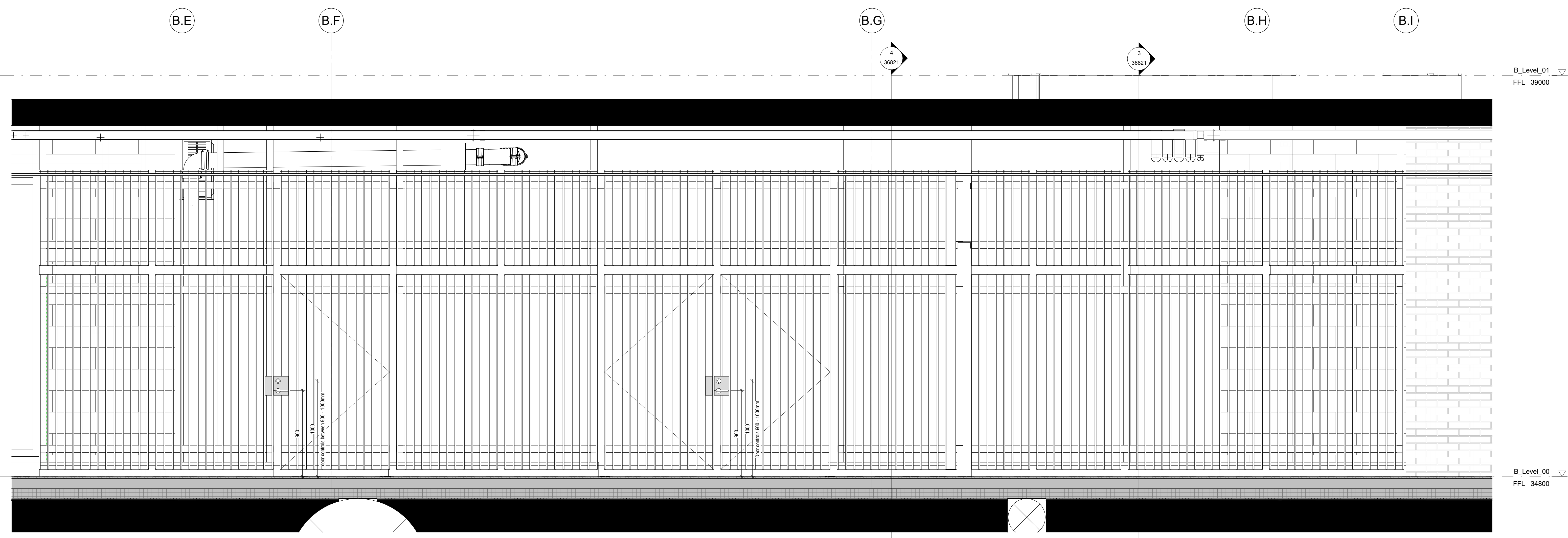
1 MWB2 - Elevation 1:20
