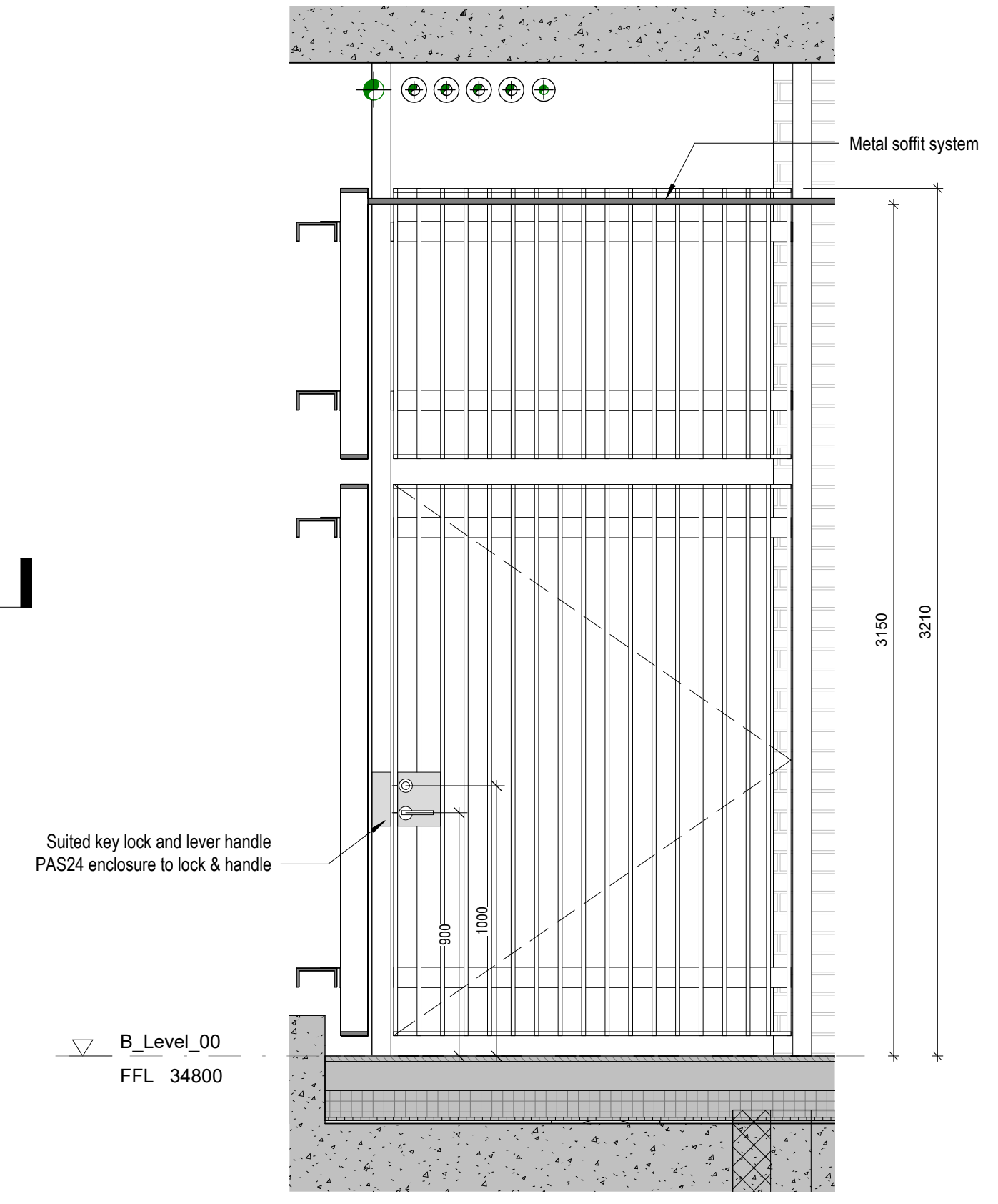
4 MWB2 - Section1 1:20
