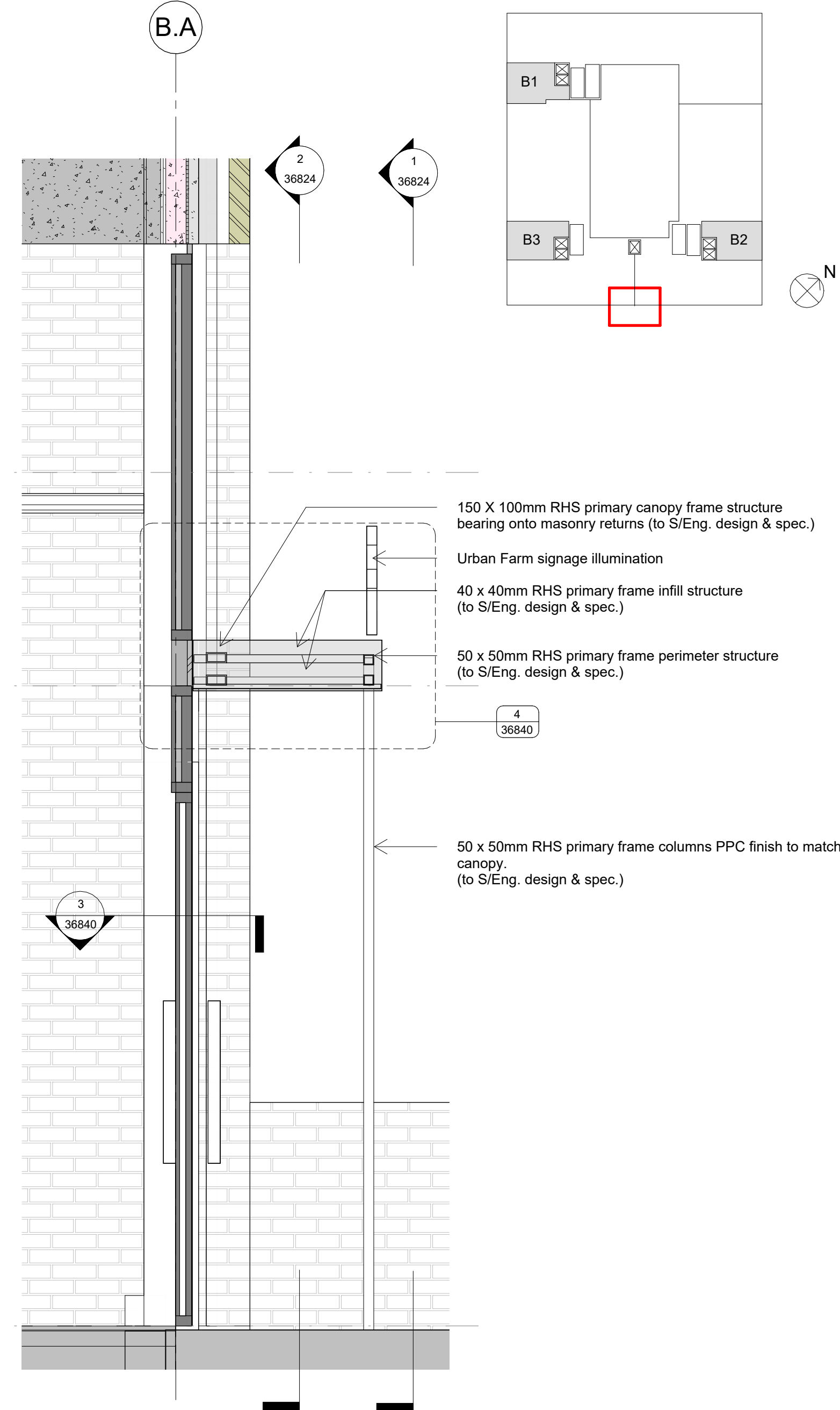
3 Cross Section Through Entrance Canopy 1: 20
