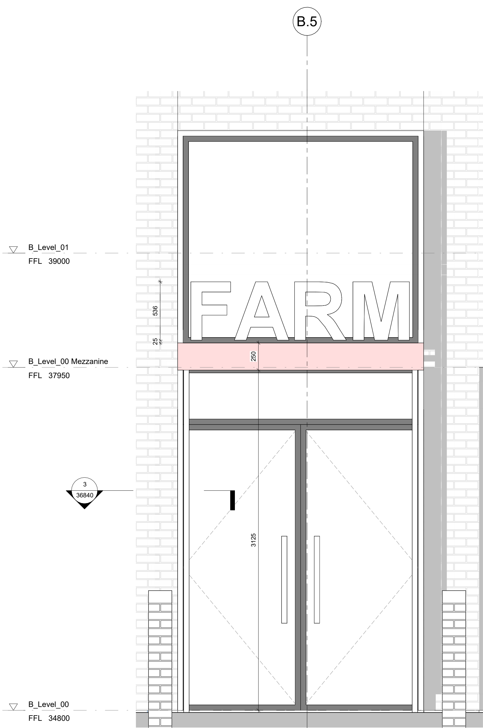
1 Elevation- Urban Farm Entrance Canopy 1: 20
