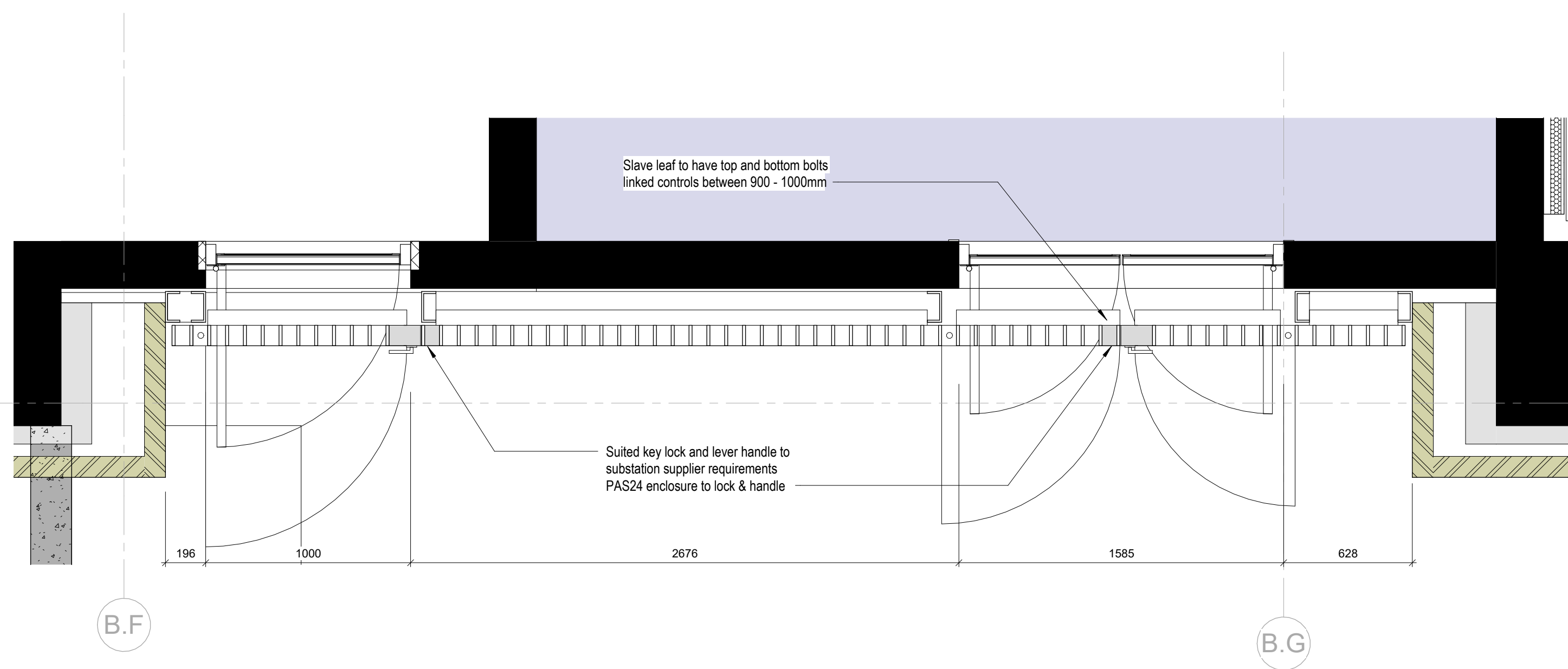
2 Cladding Bay Study 01 Plan 1:20
