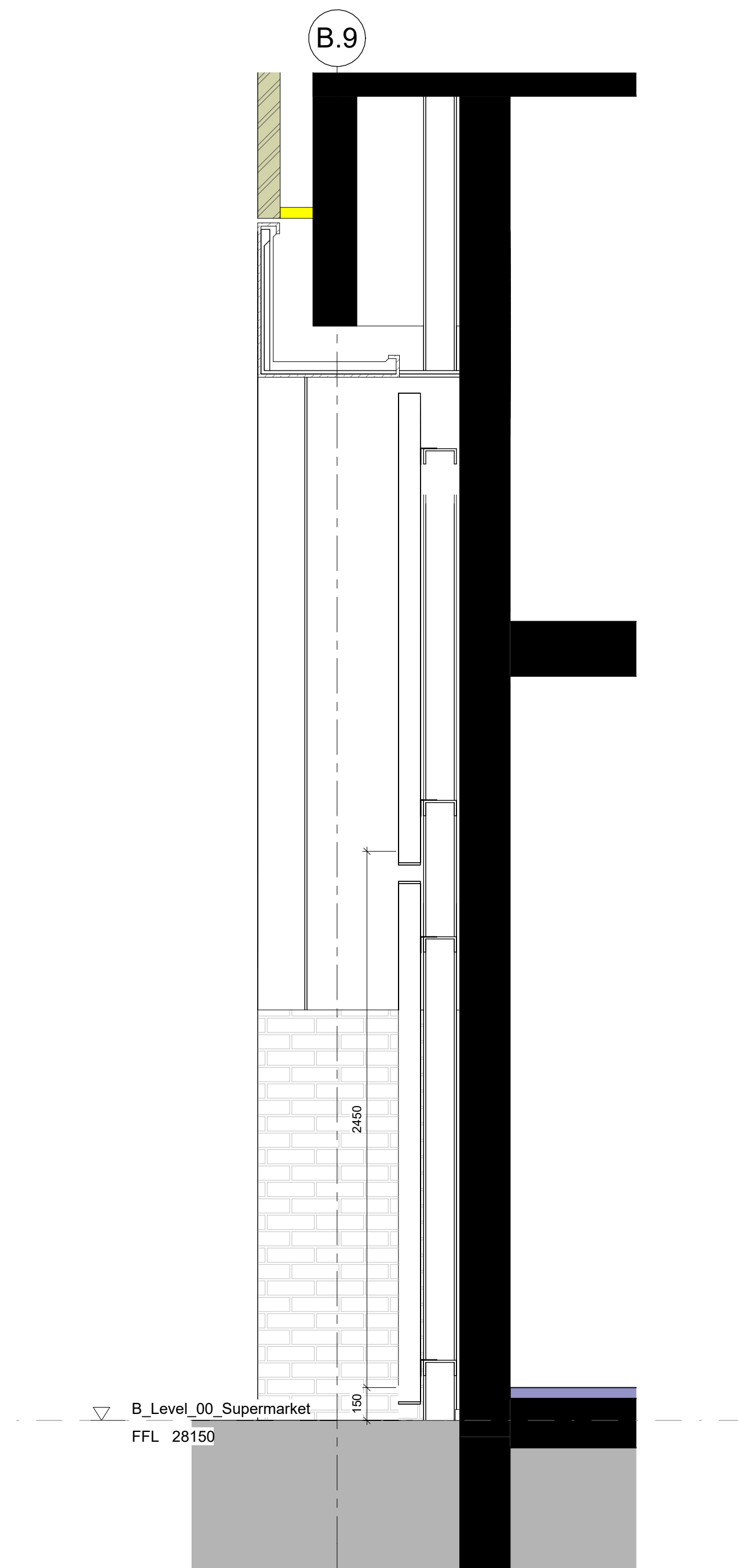
B Cladding Section B 1:20
