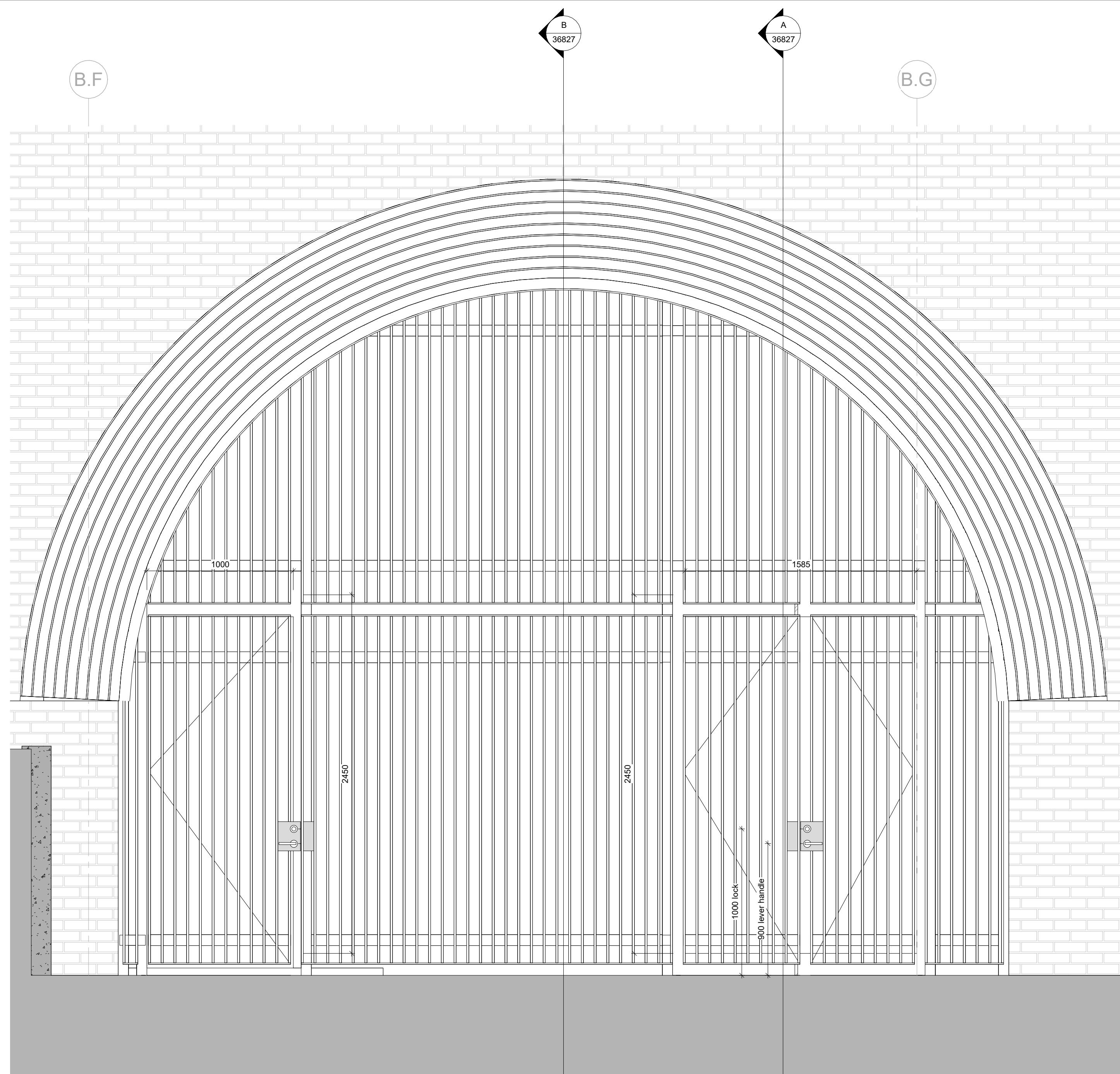
1 Cladding Bay Elevation 1:20
