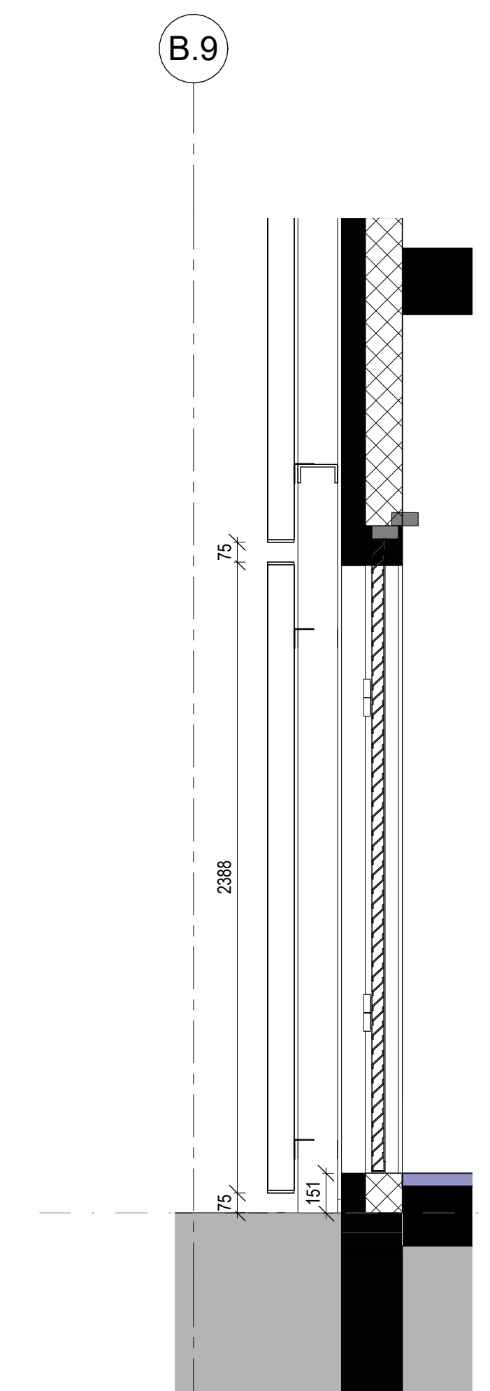
A Cladding Section A 1:20
