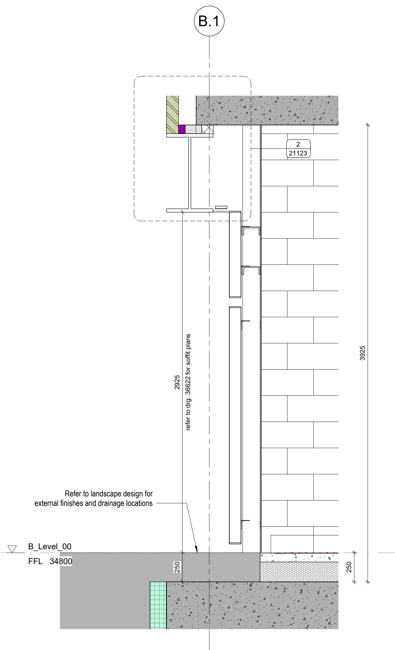
3 Cladding Bay Study 04 Section 1:20
