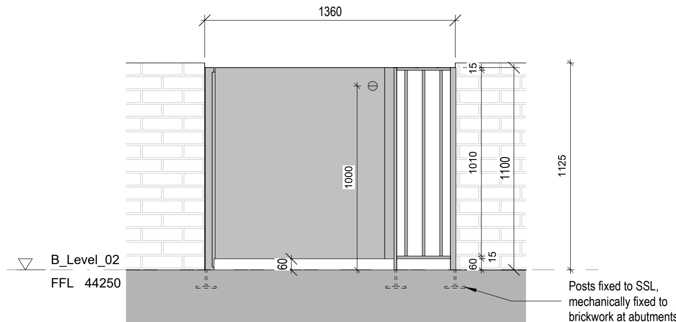
5 Metalwork Gate Lvl 02 1: 20
