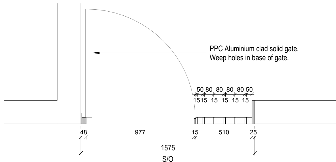
3 Metalwork Gates Plan 1: 20
