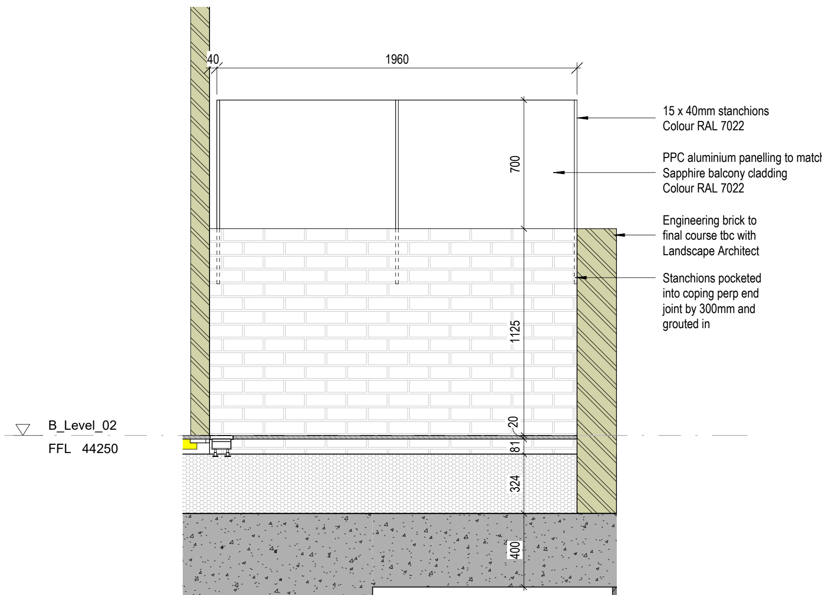
2 Metal Partition to Terraces 1: 20
