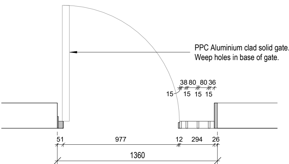
6 Metalwork Gate Plan Lvl 2 1: 20
