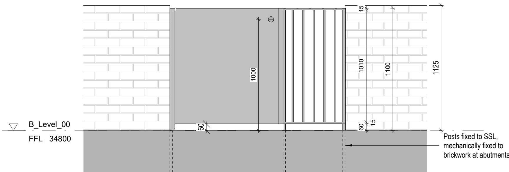
1 Metal Gate Elevation 1: 20
