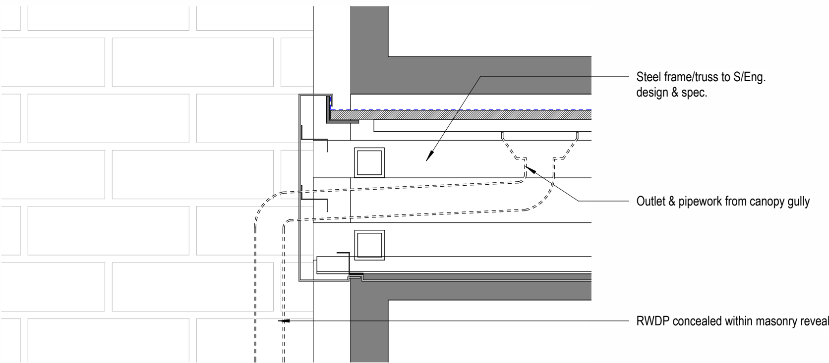
5 URBAN FARM ENTRANCE - Canopy Drainage - Edge section Copy 1:5
