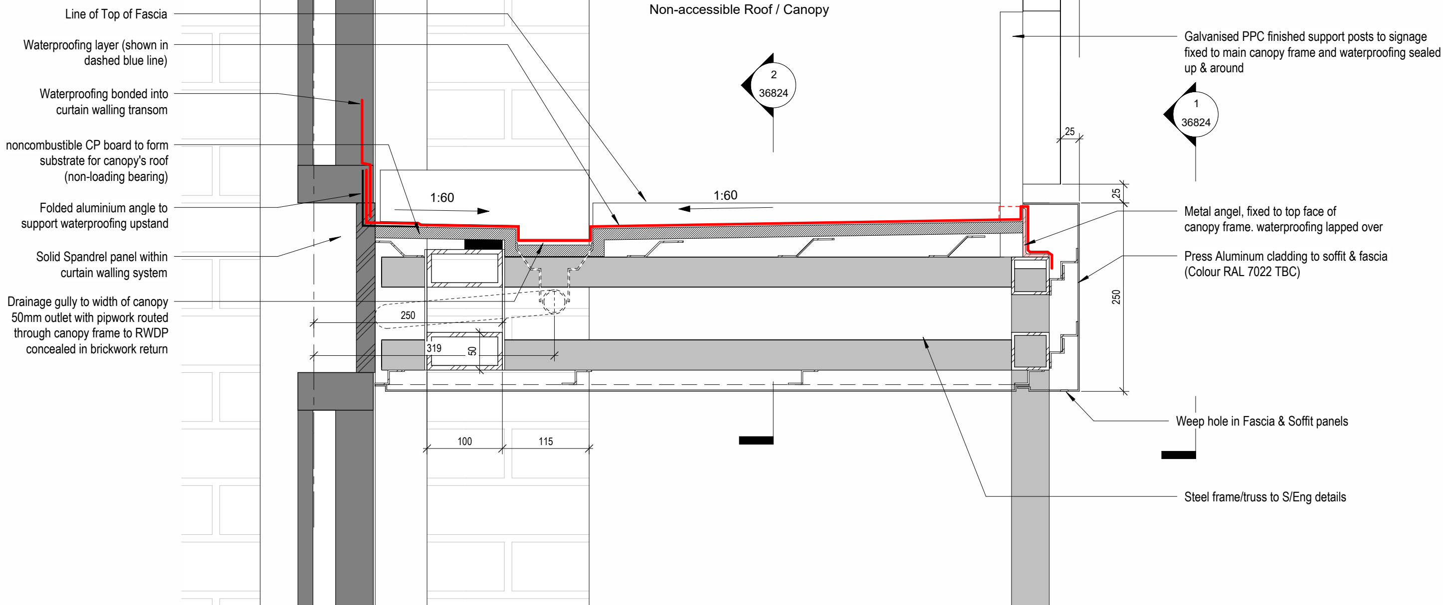
4 URBAN FARM ENTRANCE - Canopy Drainage- Cross Section 1:5
