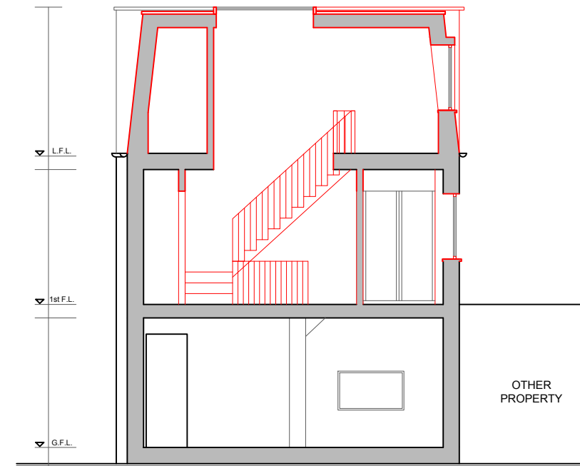
PROPOSED A-A SECTION
