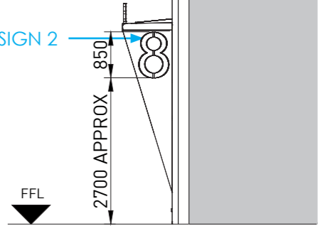
SIDE ELEVATION Scale 1:100
