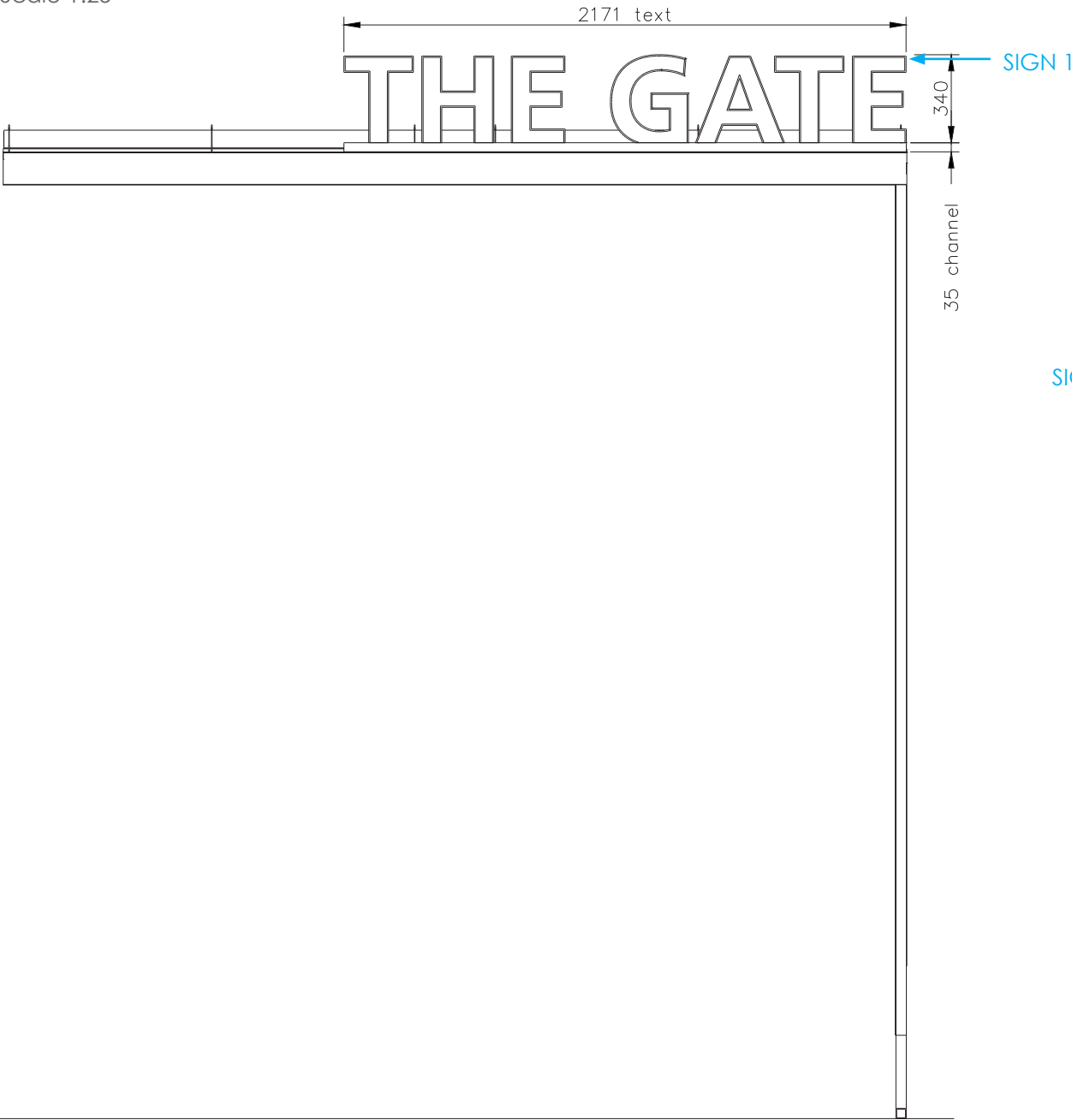
FRONT ELEVATION Scale 1:25
