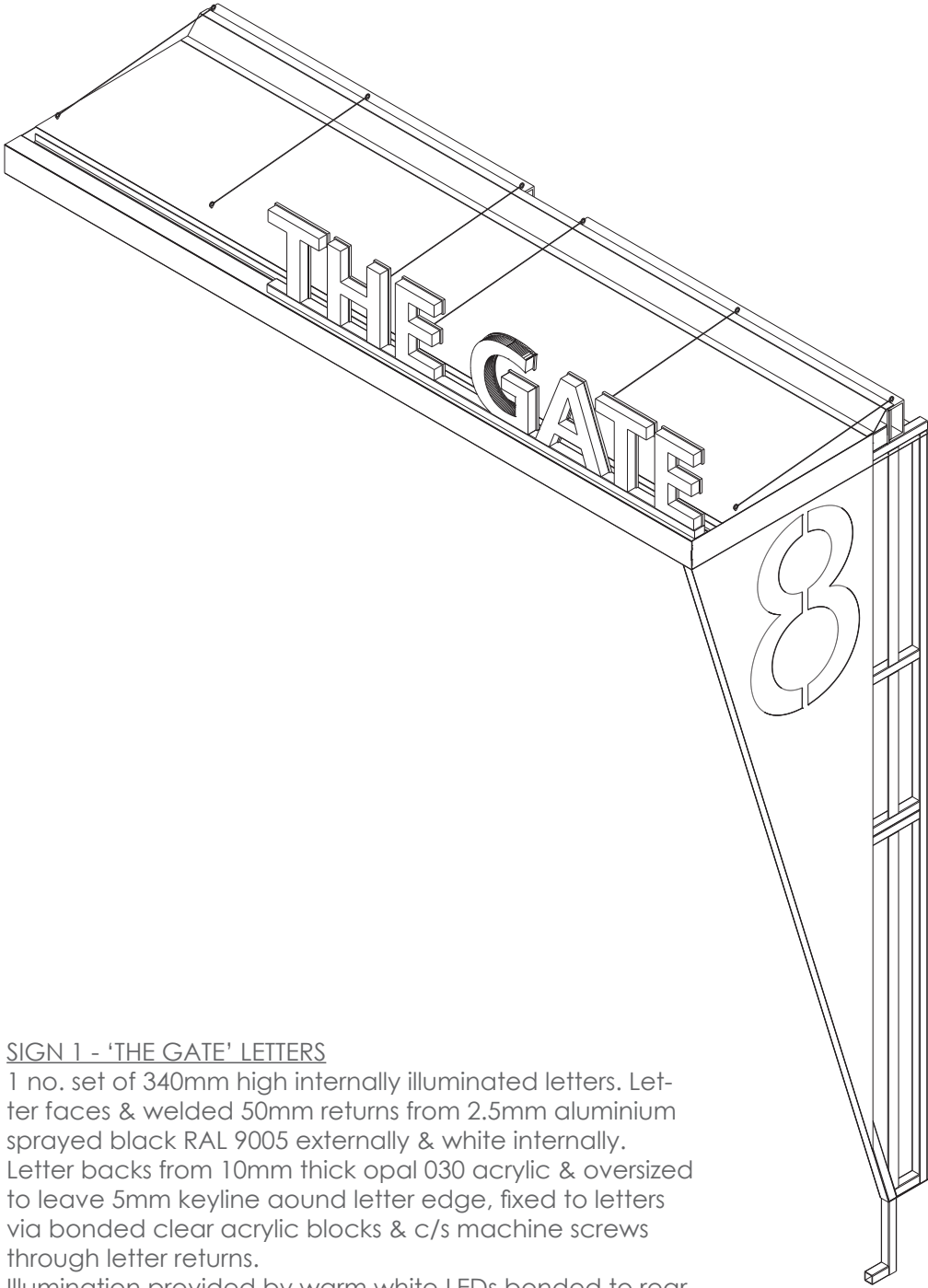
ISOMETRIC VIEW Scale 1:25
