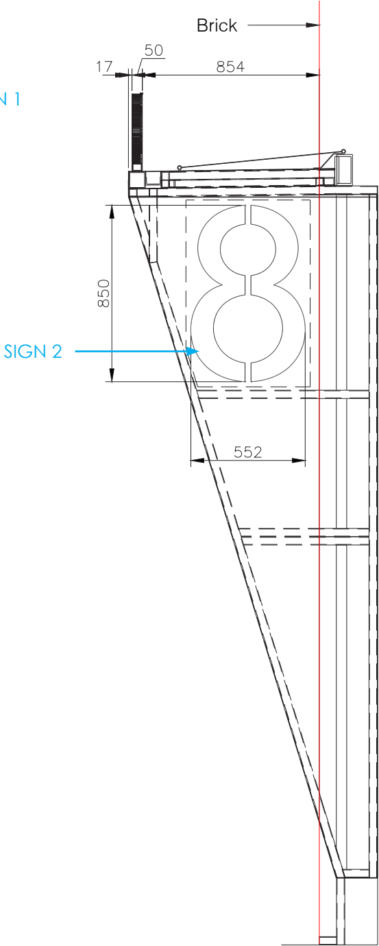
SIDE ELEVATION Scale 1:25
