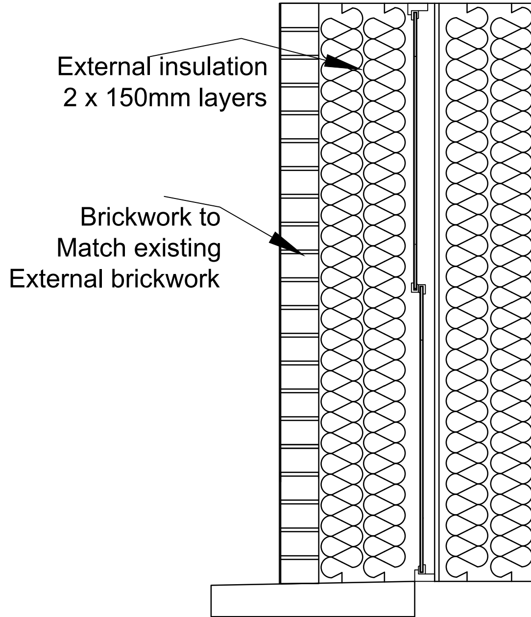
Detail - A Section Through the external window
