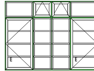
1 No. 1,995 mm x 1,475 mm Casement
