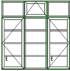
1 No. 1,480 mm x 1,480 mm Casement
