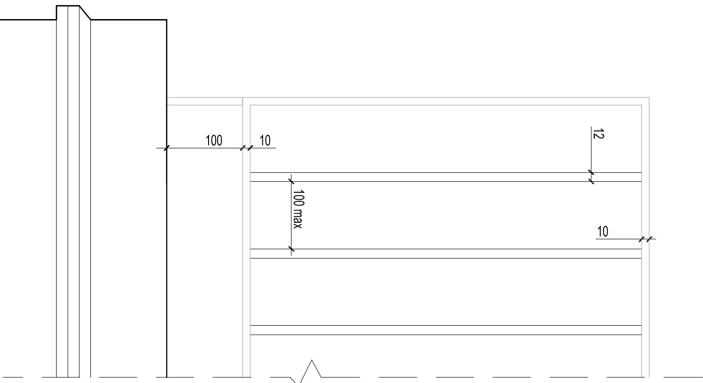
Railings Details Design based on original Victorian railings Scale 1:5
