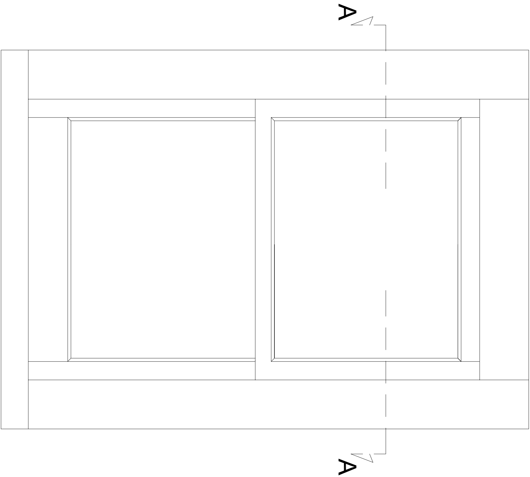
External Elevation of sliding box sash window Scale 1:5
