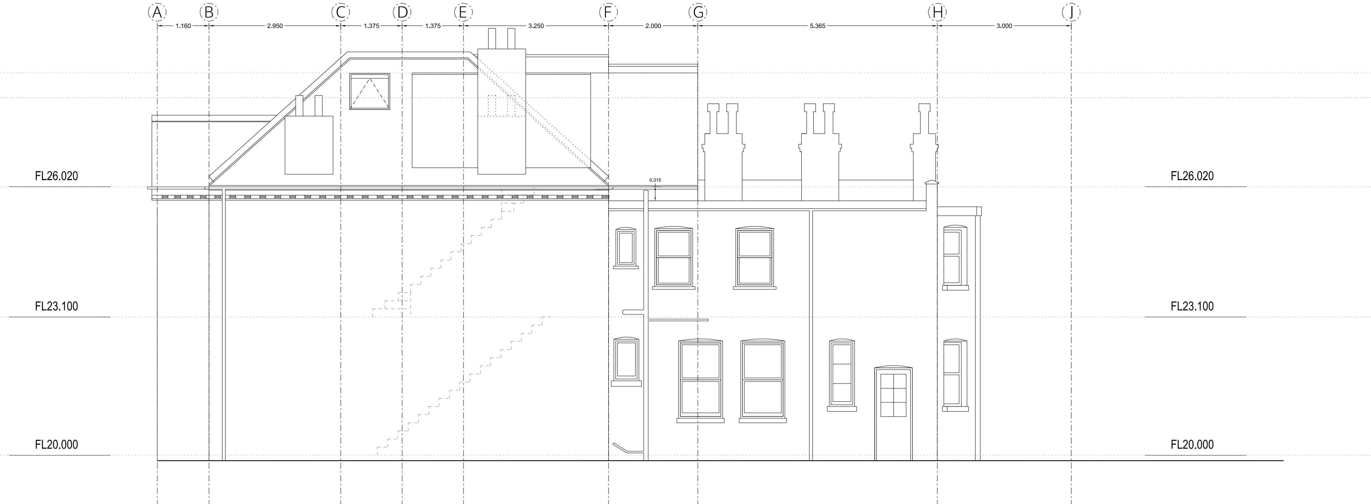
SIDE ELEVATION
