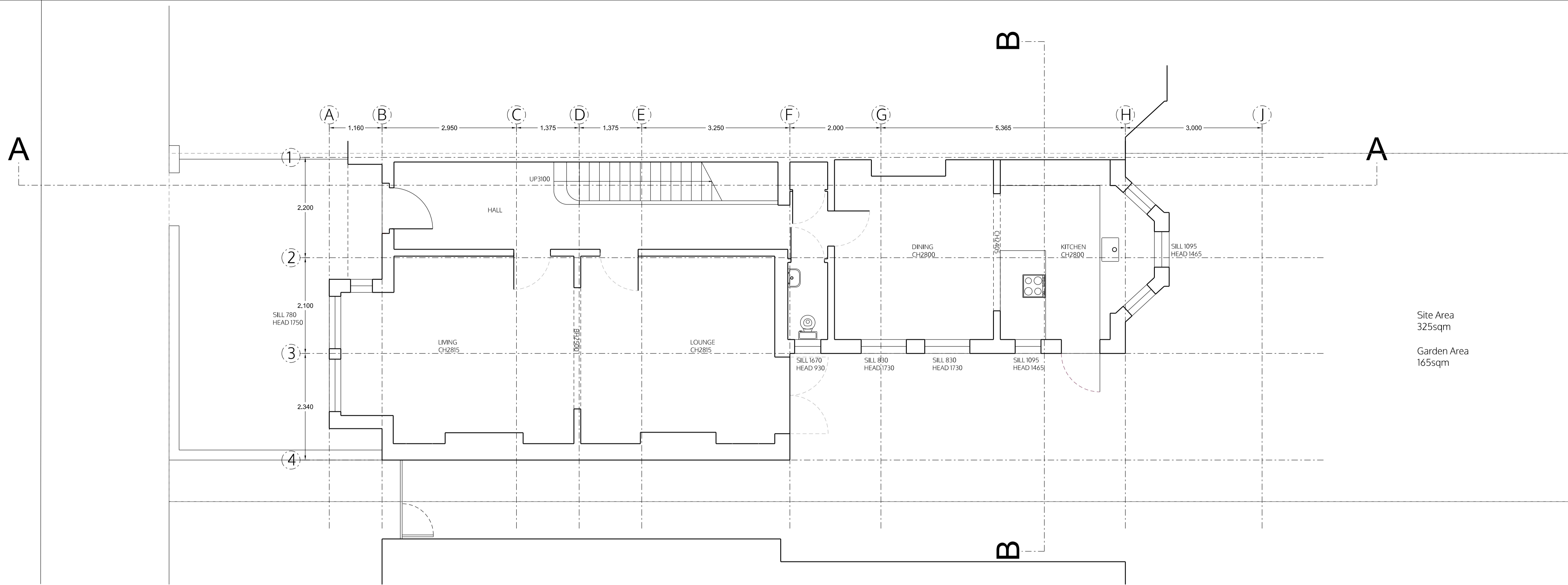
GROUND FLOOR
