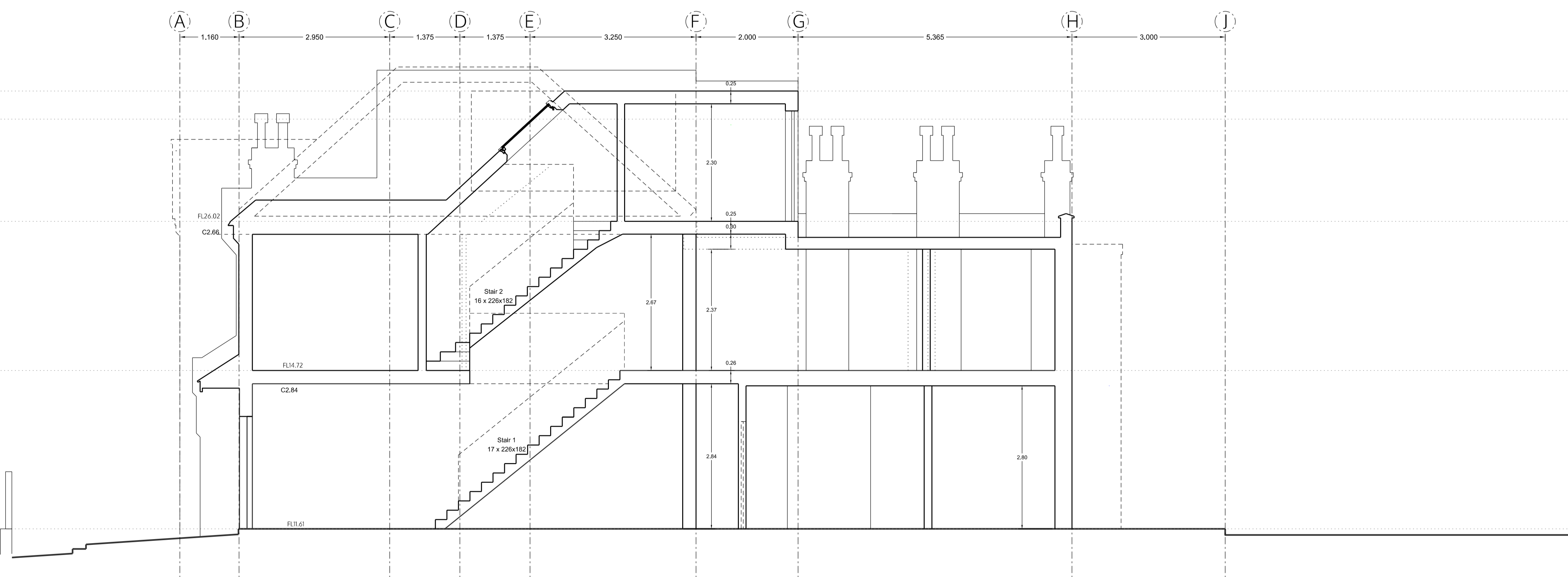
SECTION AA
