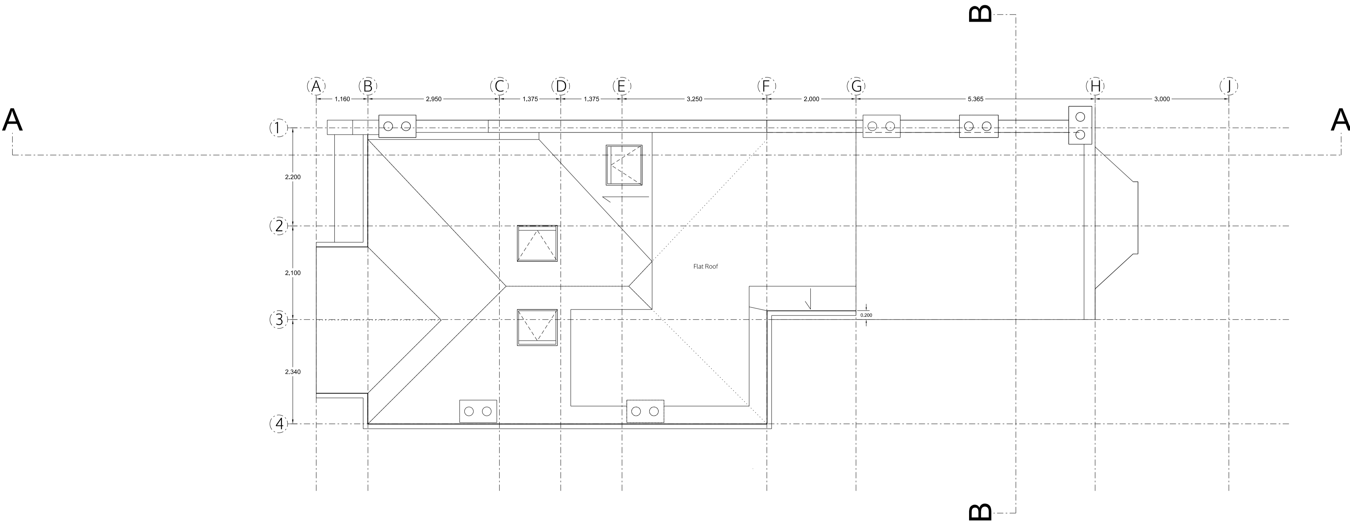
ROOF PLAN
