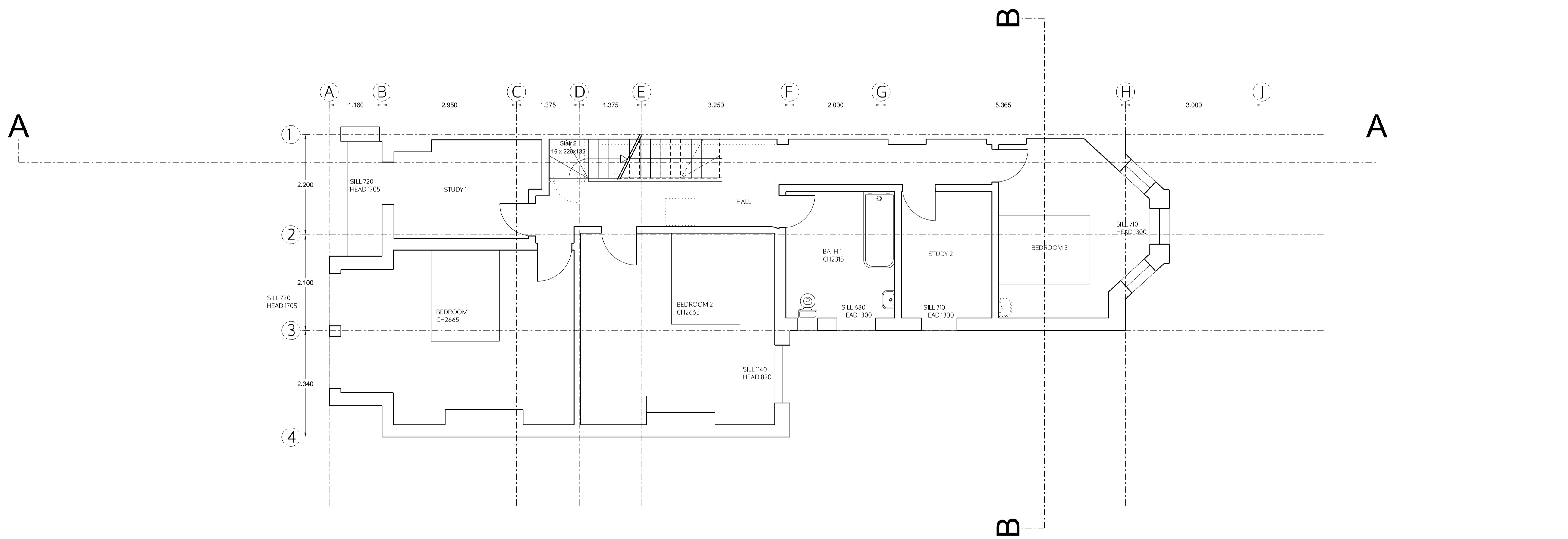
FIRST FLOOR
